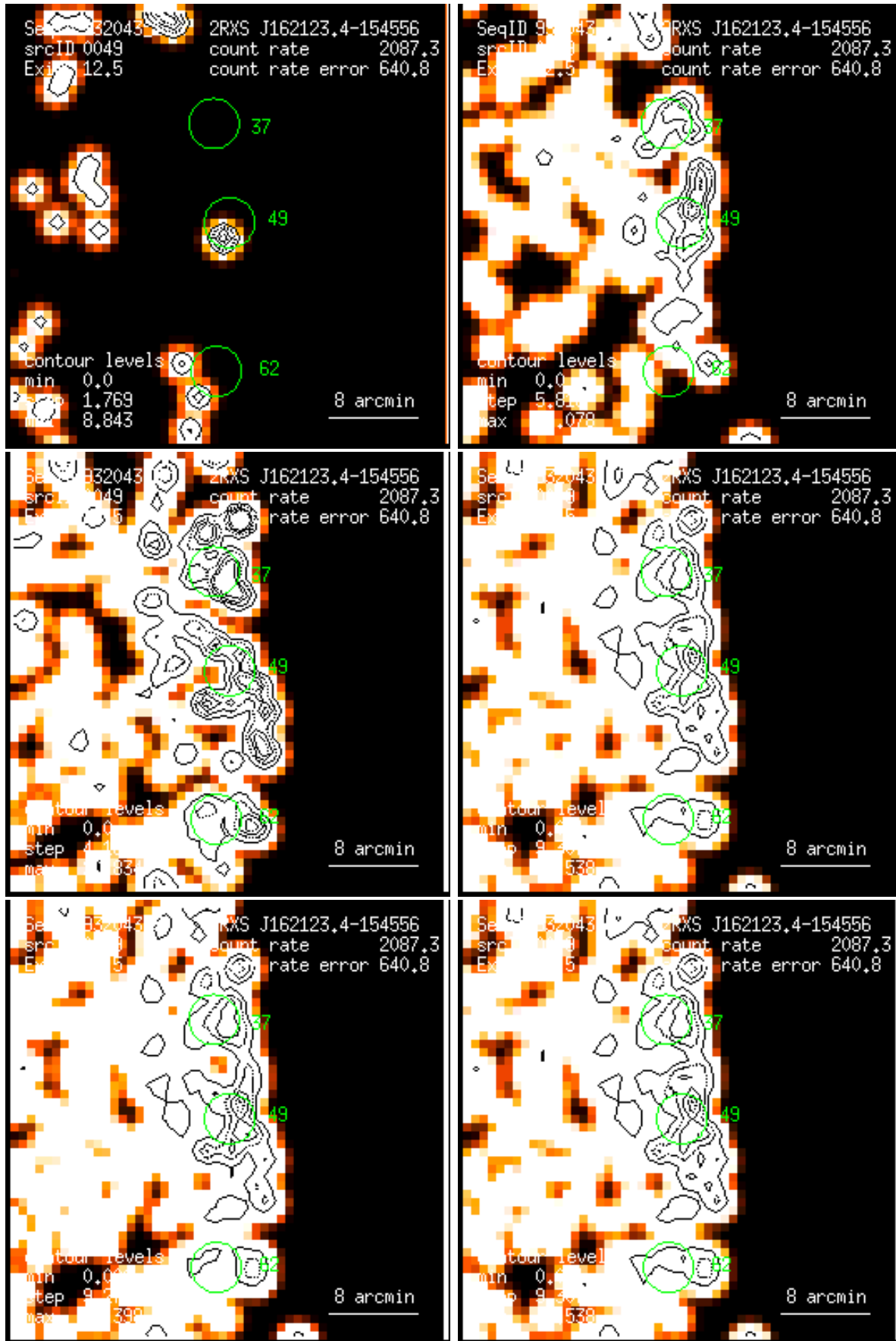
Figure 49: RASS 932043: detection 0049: band rate images, Gaussian filter: (1) PSPC channels 11 – 41, (2) 52 – 90, (3) 91 – 201, (4) 11 – 235, (5) 52 – 201, (6) 11 – 201. Broad band rates in counts/ks. Band rate contour levels in counts/ks/arcmin 2 .
