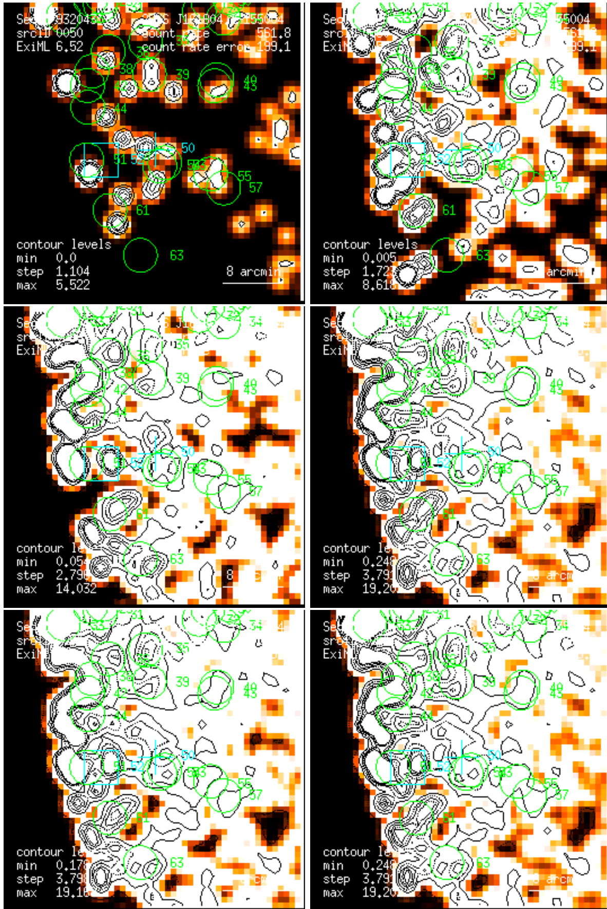
Figure 50: RASS 932043: detection 0050: band rate images, Gaussian filter: (1) PSPC channels 11 – 41, (2) 52 – 90, (3) 91 – 201, (4) 11 – 235, (5) 52 – 201, (6) 11 – 201. Broad band rates in counts/ks. Band rate contour levels in counts/ks/arcmin 2 .
