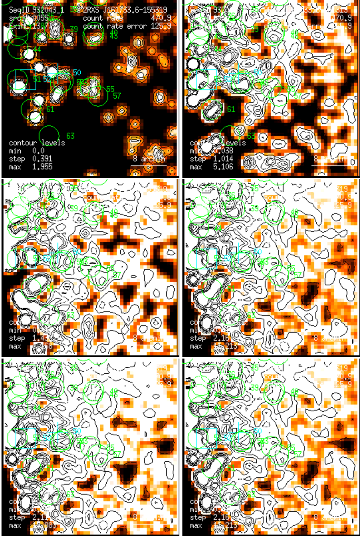
Figure 55: RASS 932043: detection 0055: band rate images, Gaussian filter: (1) PSPC channels 11 – 41, (2) 52 – 90, (3) 91 – 201, (4) 11 – 235, (5) 52 – 201, (6) 11 – 201. Broad band rates in counts/ks. Band rate contour levels in counts/ks/arcmin 2 .
