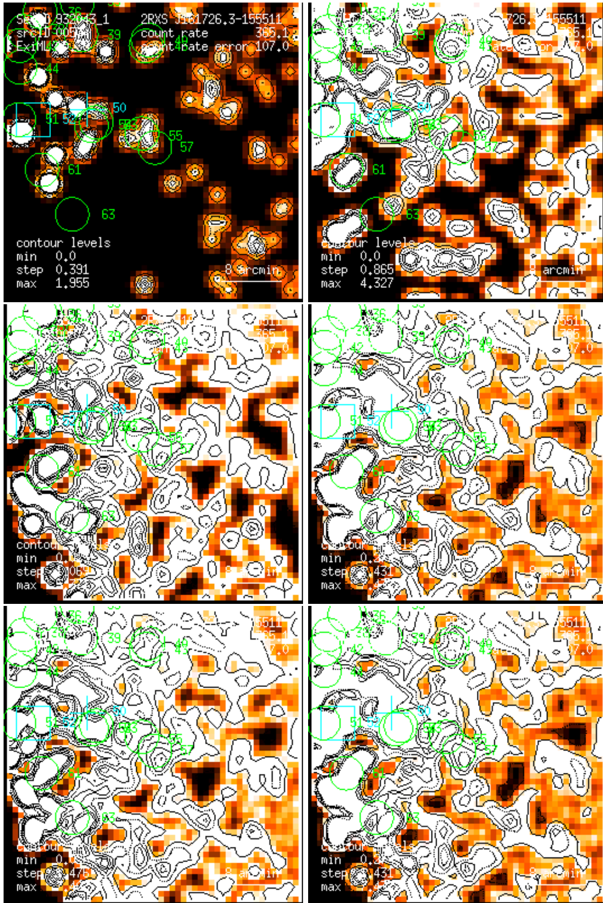
Figure 57: RASS 932043: detection 0057: band rate images, Gaussian filter: (1) PSPC channels 11 – 41, (2) 52 – 90, (3) 91 – 201, (4) 11 – 235, (5) 52 – 201, (6) 11 – 201. Broad band rates in counts/ks. Band rate contour levels in counts/ks/arcmin 2 .
