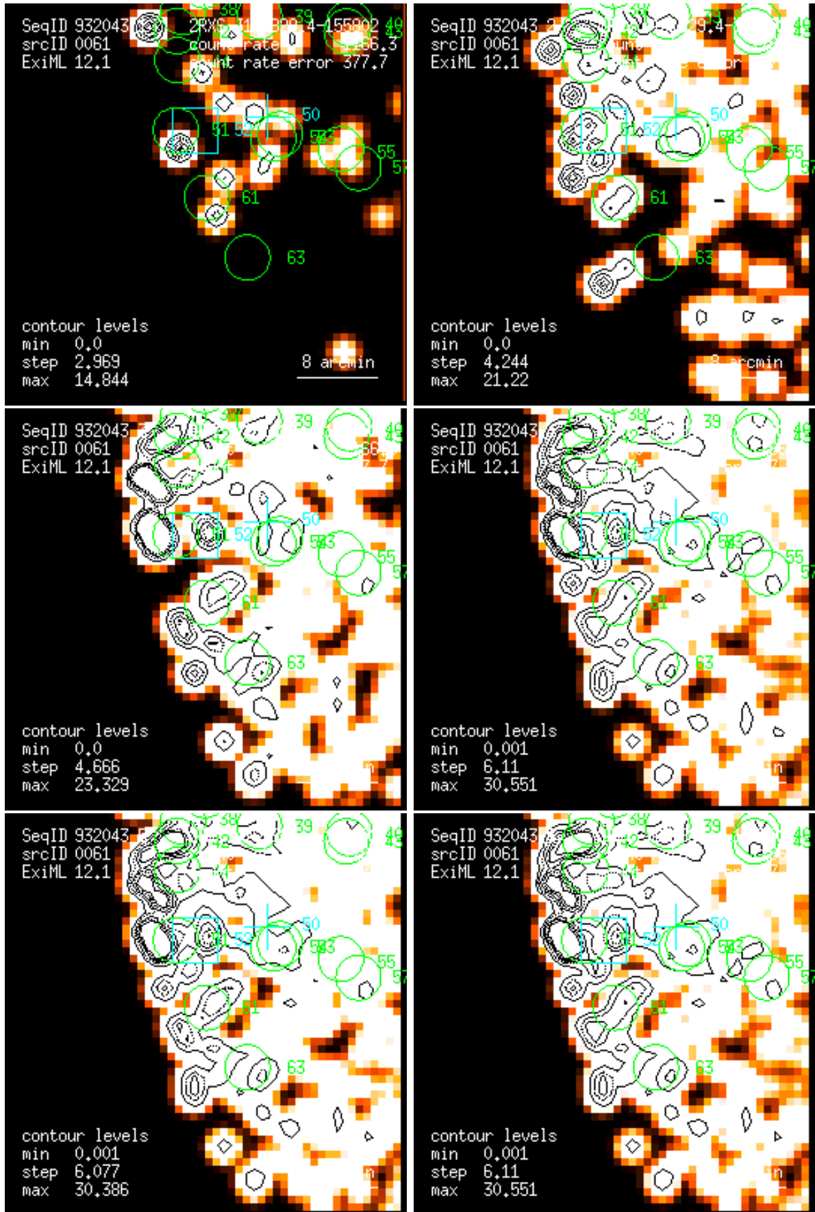
Figure 61: RASS 932043: detection 0061: band rate images, Gaussian filter: (1) PSPC channels 11 – 41, (2) 52 – 90, (3) 91 – 201, (4) 11 – 235, (5) 52 – 201, (6) 11 – 201. Broad band rates in counts/ks. Band rate contour levels in counts/ks/arcmin 2 .
