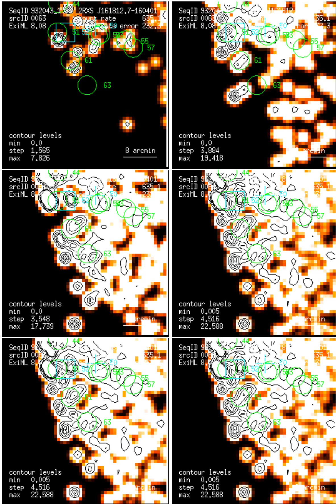
Figure 63: RASS 932043: detection 0063: band rate images, Gaussian filter: (1) PSPC channels 11 – 41, (2) 52 – 90, (3) 91 – 201, (4) 11 – 235, (5) 52 – 201, (6) 11 – 201. Broad band rates in counts/ks. Band rate contour levels in counts/ks/arcmin 2 .
