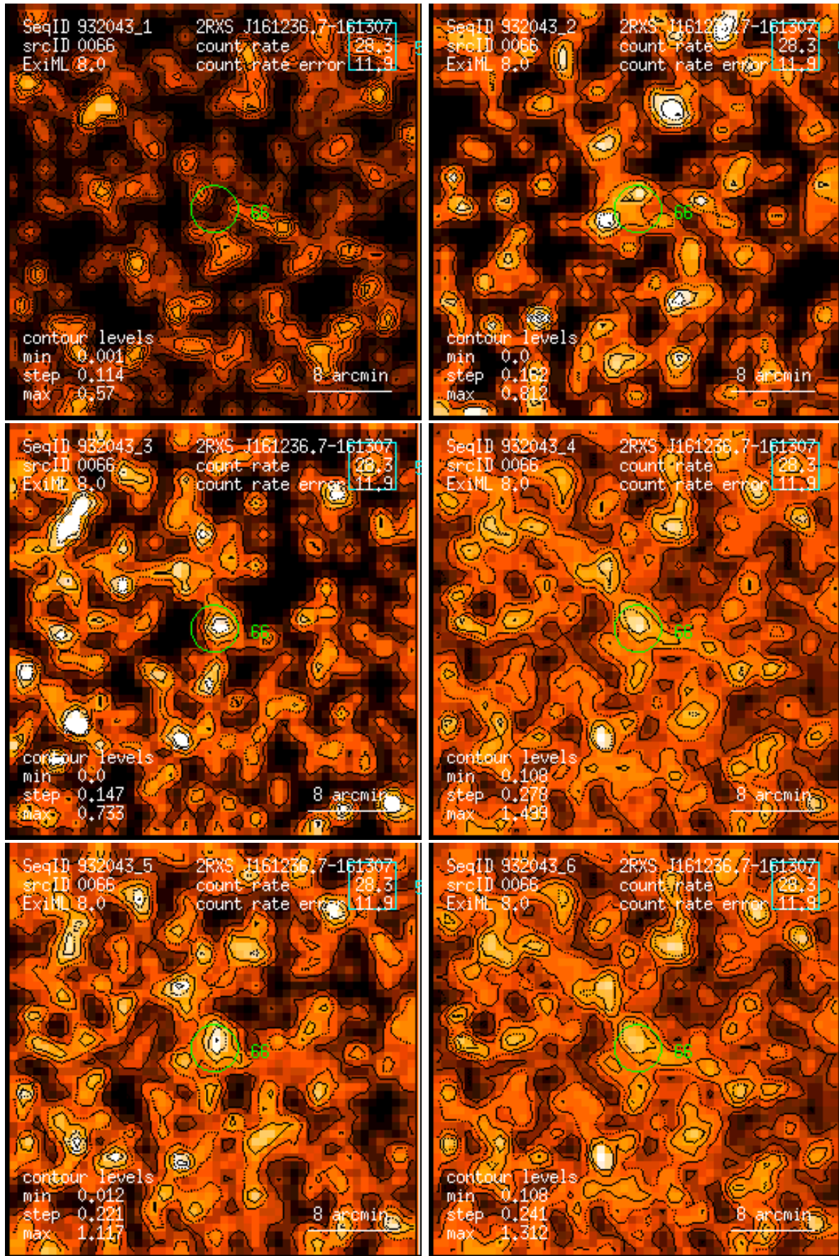
Figure 66: RASS 932043: detection 0066: band rate images, Gaussian filter: (1) PSPC channels 11 – 41, (2) 52 – 90, (3) 91 – 201, (4) 11 – 235, (5) 52 – 201, (6) 11 – 201. Broad band rates in counts/ks. Band rate contour levels in counts/ks/arcmin 2 .
