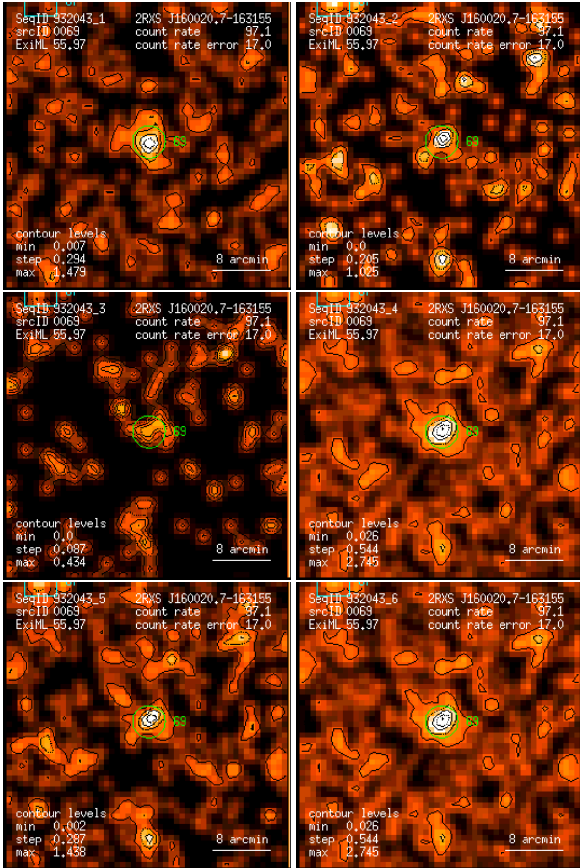
Figure 69: RASS 932043: detection 0069: band rate images, Gaussian filter: (1) PSPC channels 11 – 41, (2) 52 – 90, (3) 91 – 201, (4) 11 – 235, (5) 52 – 201, (6) 11 – 201. Broad band rates in counts/ks. Band rate contour levels in counts/ks/arcmin 2 .
