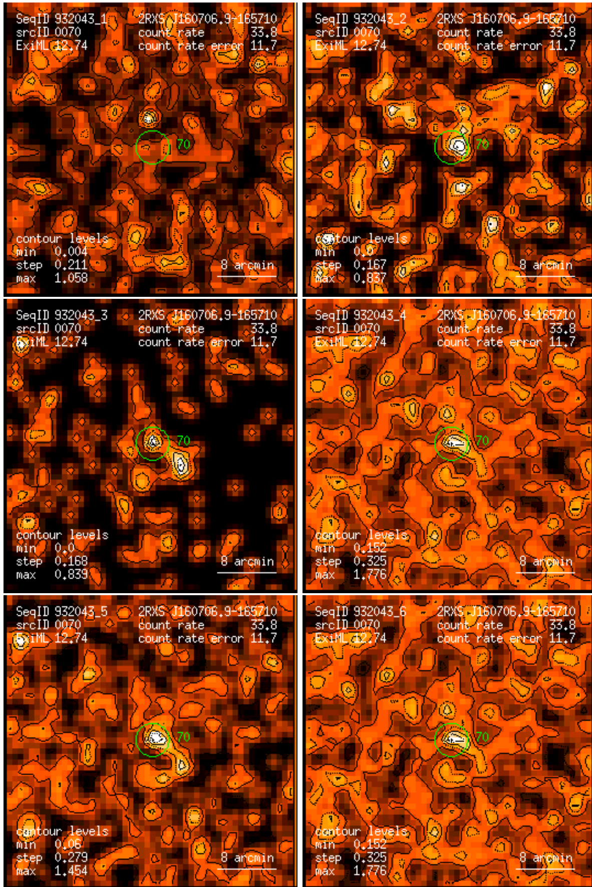
Figure 70: RASS 932043: detection 0070: band rate images, Gaussian filter: (1) PSPC channels 11 – 41, (2) 52 – 90, (3) 91 – 201, (4) 11 – 235, (5) 52 – 201, (6) 11 – 201. Broad band rates in counts/ks. Band rate contour levels in counts/ks/arcmin 2 .
