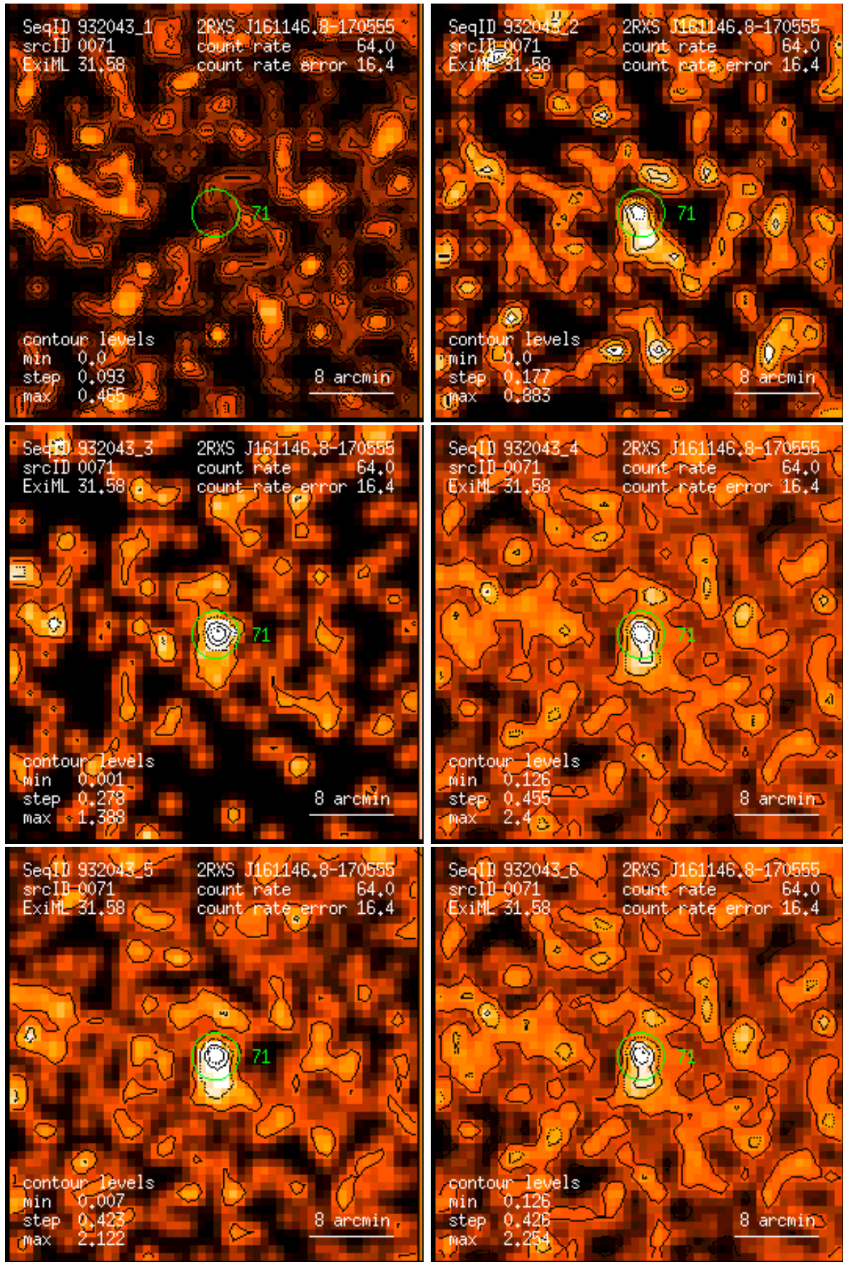
Figure 71: RASS 932043: detection 0071: band rate images, Gaussian filter: (1) PSPC channels 11 – 41, (2) 52 – 90, (3) 91 – 201, (4) 11 – 235, (5) 52 – 201, (6) 11 – 201. Broad band rates in counts/ks. Band rate contour levels in counts/ks/arcmin 2 .
