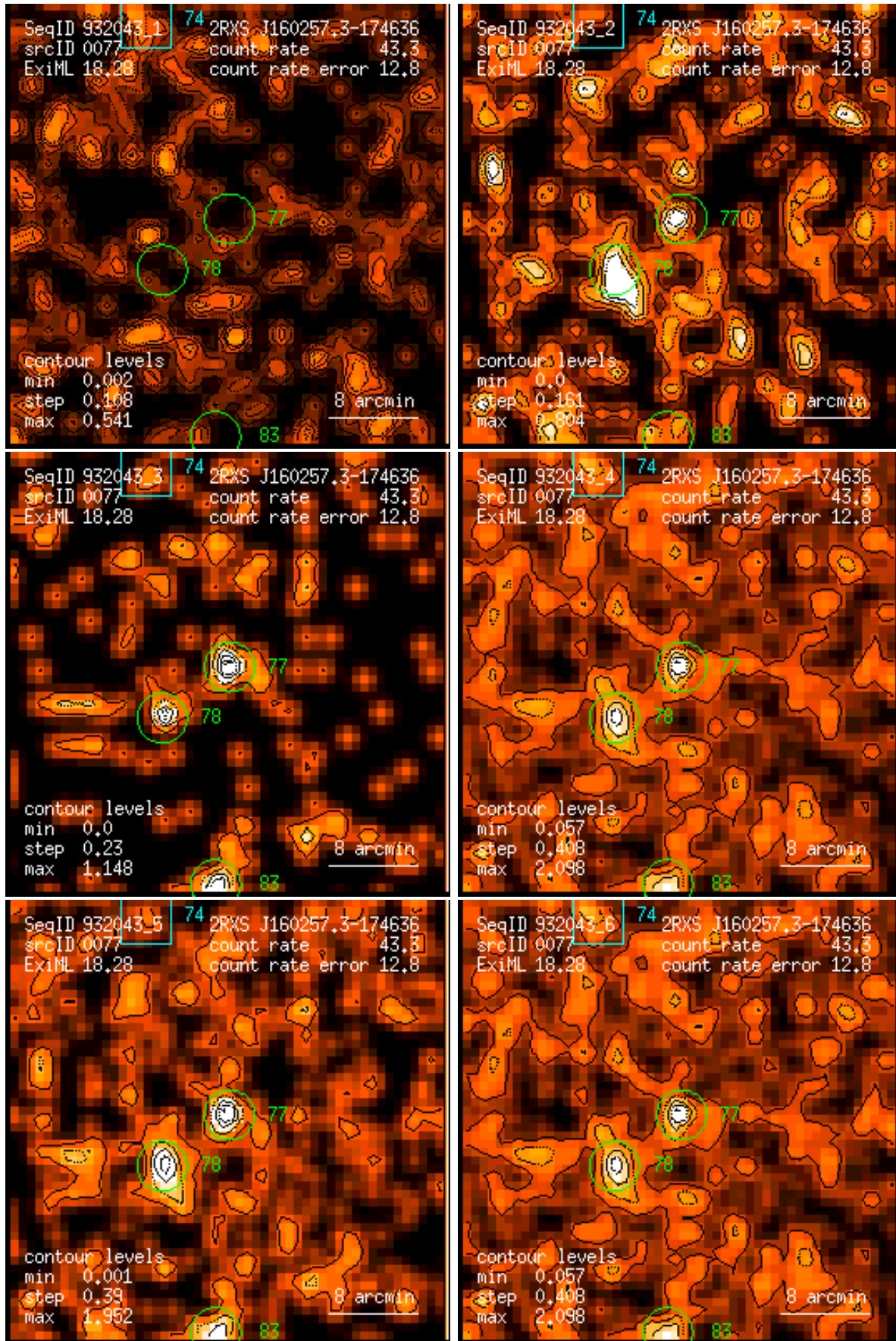
Figure 77: RASS 932043: detection 0077: band rate images, Gaussian filter: (1) PSPC channels 11 – 41, (2) 52 – 90, (3) 91 – 201, (4) 11 – 235, (5) 52 – 201, (6) 11 – 201. Broad band rates in counts/ks. Band rate contour levels in counts/ks/arcmin 2 .
