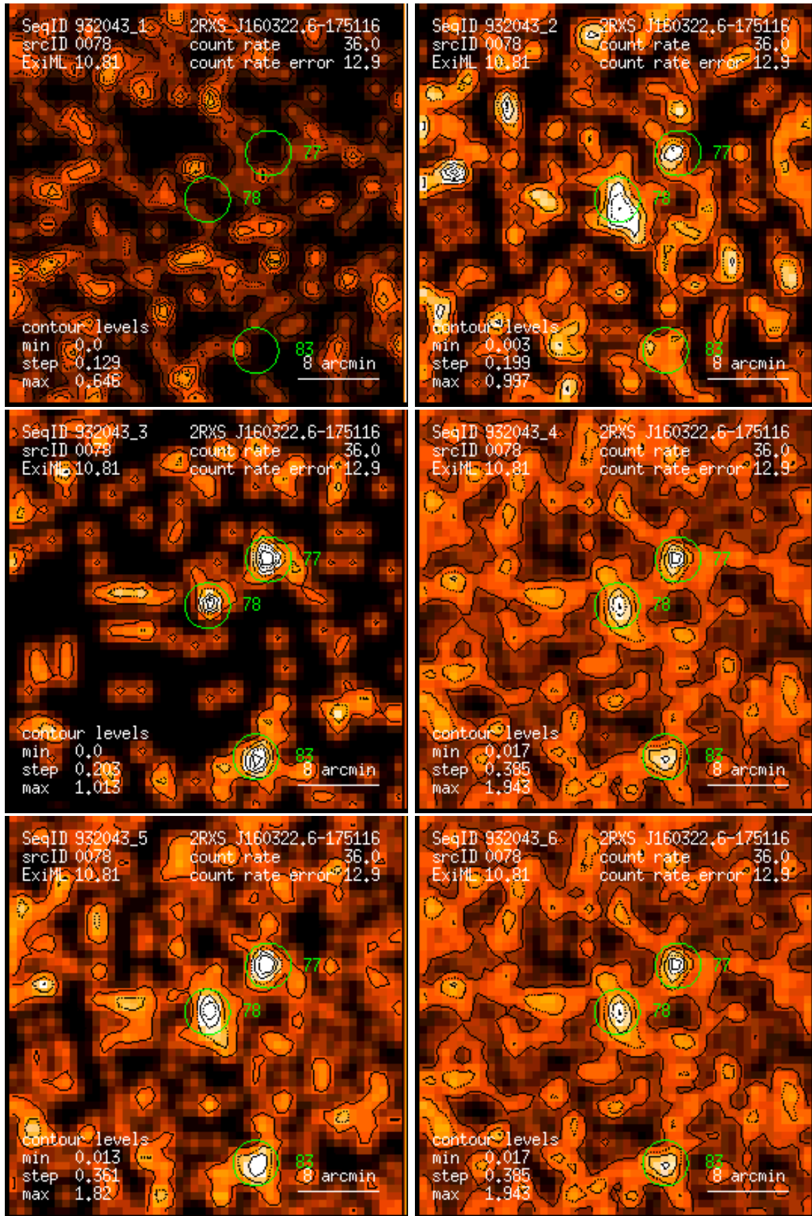
Figure 78: RASS 932043: detection 0078: band rate images, Gaussian filter: (1) PSPC channels 11 – 41, (2) 52 – 90, (3) 91 – 201, (4) 11 – 235, (5) 52 – 201, (6) 11 – 201. Broad band rates in counts/ks. Band rate contour levels in counts/ks/arcmin 2 .
