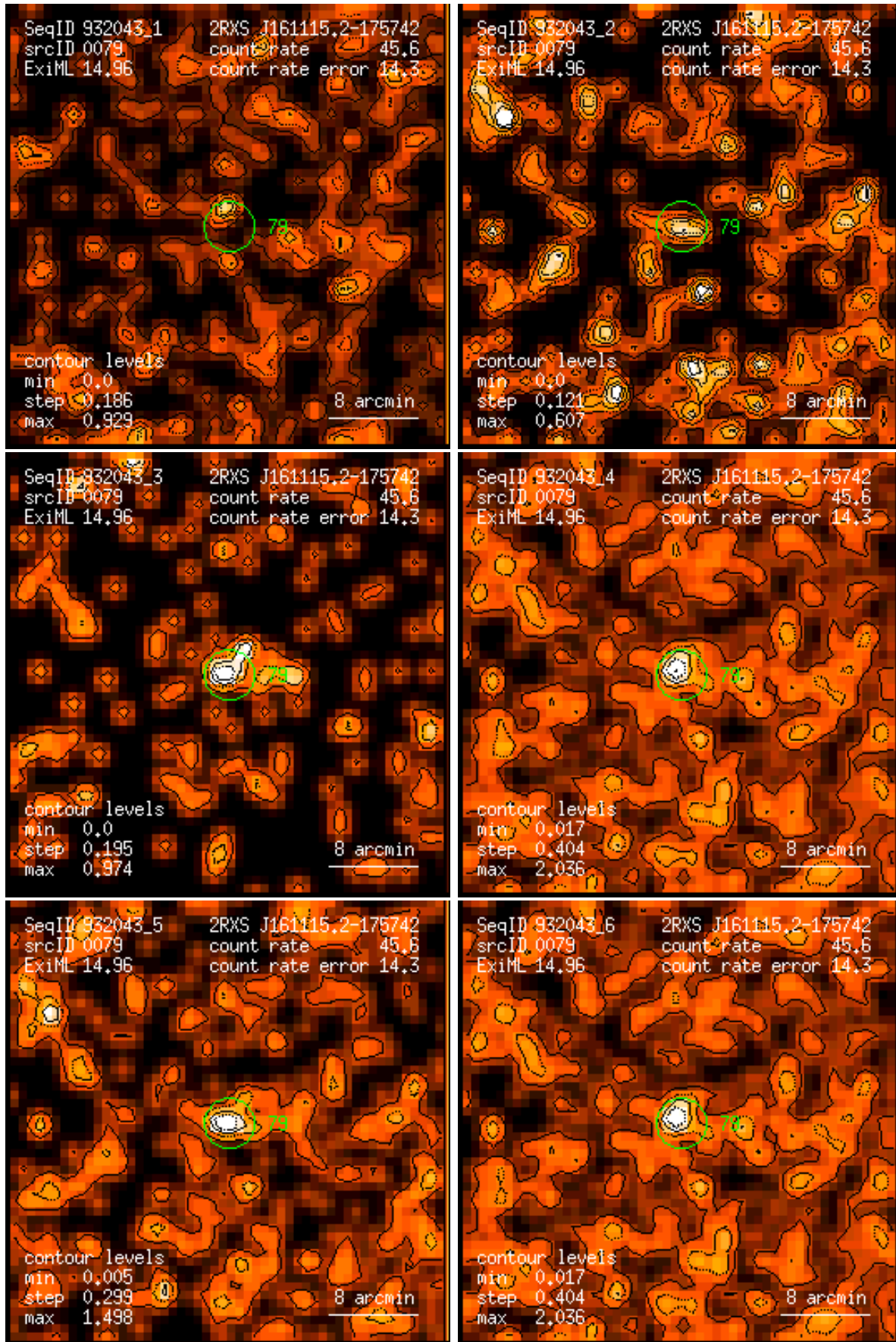
Figure 79: RASS 932043: detection 0079: band rate images, Gaussian filter: (1) PSPC channels 11 – 41, (2) 52 – 90, (3) 91 – 201, (4) 11 – 235, (5) 52 – 201, (6) 11 – 201. Broad band rates in counts/ks. Band rate contour levels in counts/ks/arcmin 2 .
