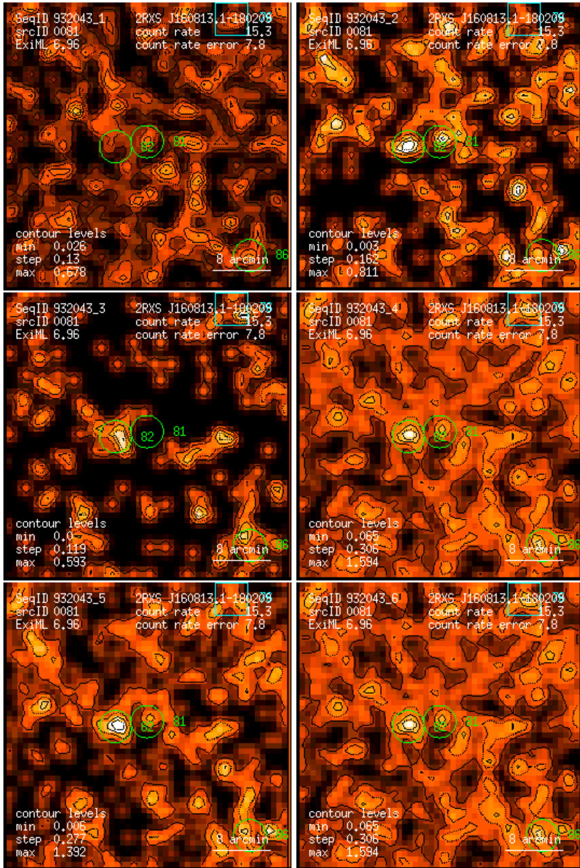
Figure 81: RASS 932043: detection 0081: band rate images, Gaussian filter: (1) PSPC channels 11 – 41, (2) 52 – 90, (3) 91 – 201, (4) 11 – 235, (5) 52 – 201, (6) 11 – 201. Broad band rates in counts/ks. Band rate contour levels in counts/ks/arcmin 2 .
