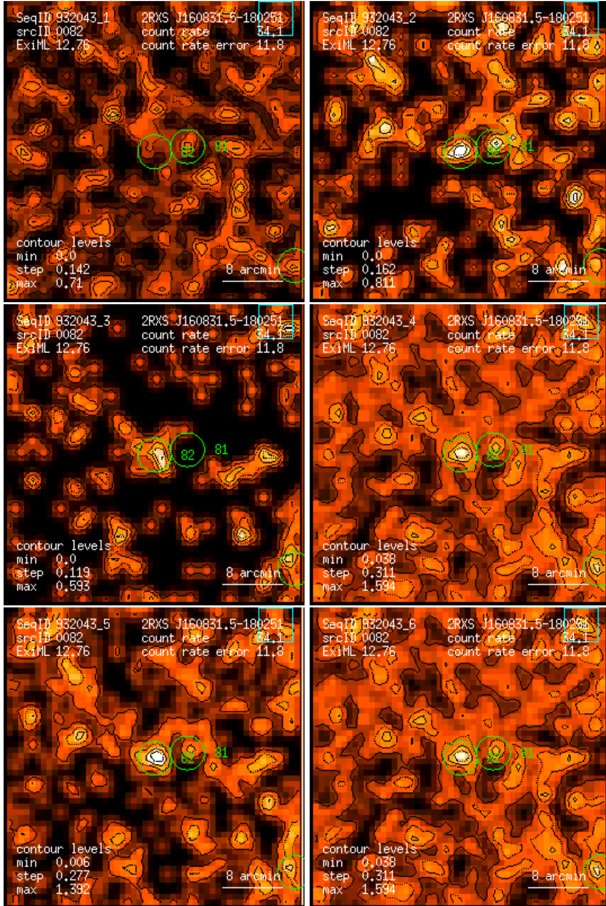
Figure 82: RASS 932043: detection 0082: band rate images, Gaussian filter: (1) PSPC channels 11 – 41, (2) 52 – 90, (3) 91 – 201, (4) 11 – 235, (5) 52 – 201, (6) 11 – 201. Broad band rates in counts/ks. Band rate contour levels in counts/ks/arcmin 2 .
