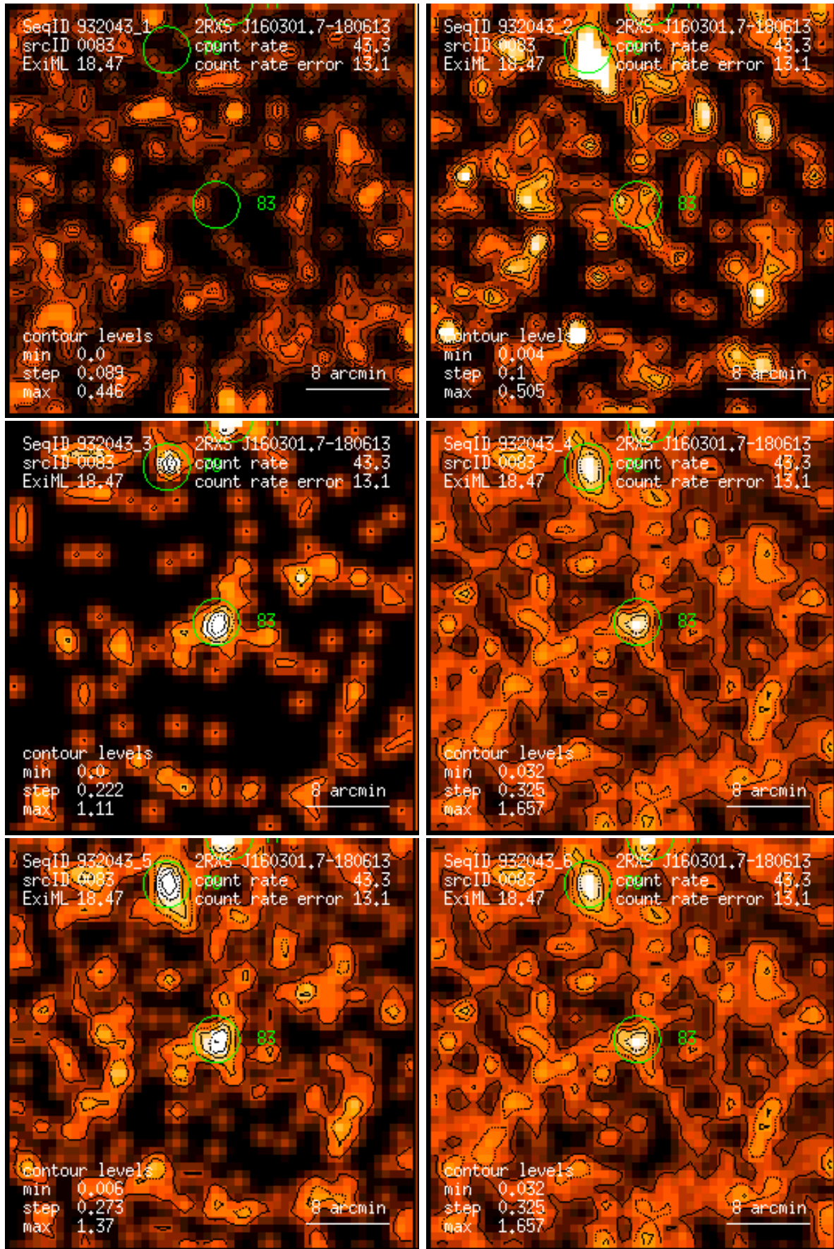
Figure 83: RASS 932043: detection 0083: band rate images, Gaussian filter: (1) PSPC channels 11 – 41, (2) 52 – 90, (3) 91 – 201, (4) 11 – 235, (5) 52 – 201, (6) 11 – 201. Broad band rates in counts/ks. Band rate contour levels in counts/ks/arcmin 2 .
