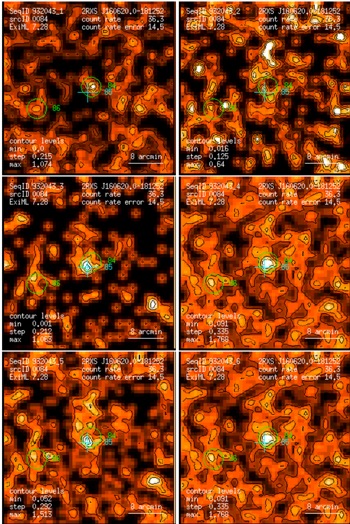
Figure 84: RASS 932043: detection 0084: band rate images, Gaussian filter: (1) PSPC channels 11 – 41, (2) 52 – 90, (3) 91 – 201, (4) 11 – 235, (5) 52 – 201, (6) 11 – 201. Broad band rates in counts/ks. Band rate contour levels in counts/ks/arcmin 2 .
