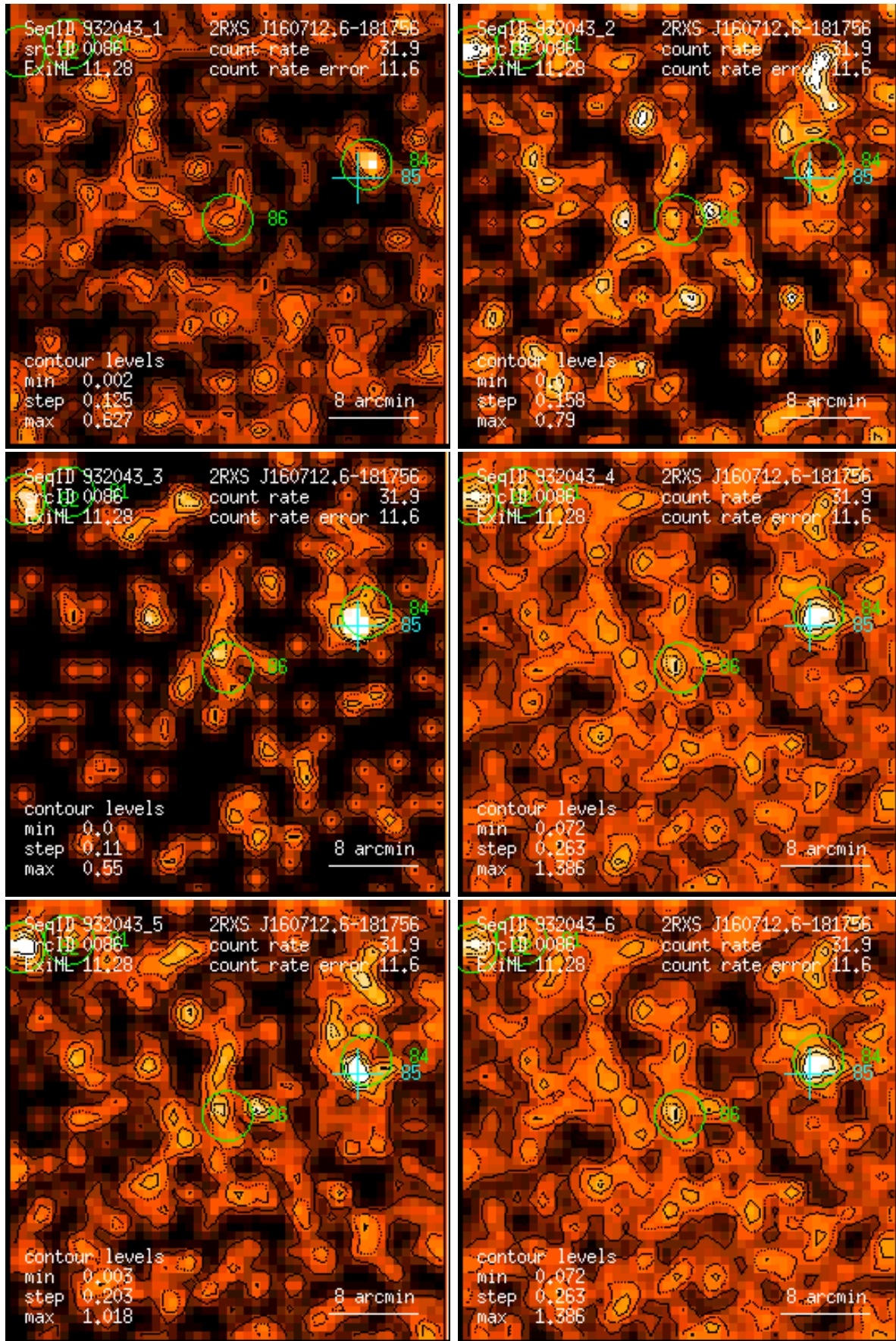
Figure 86: RASS 932043: detection 0086: band rate images, Gaussian filter: (1) PSPC channels 11 – 41, (2) 52 – 90, (3) 91 – 201, (4) 11 – 235, (5) 52 – 201, (6) 11 – 201. Broad band rates in counts/ks. Band rate contour levels in counts/ks/arcmin 2 .
