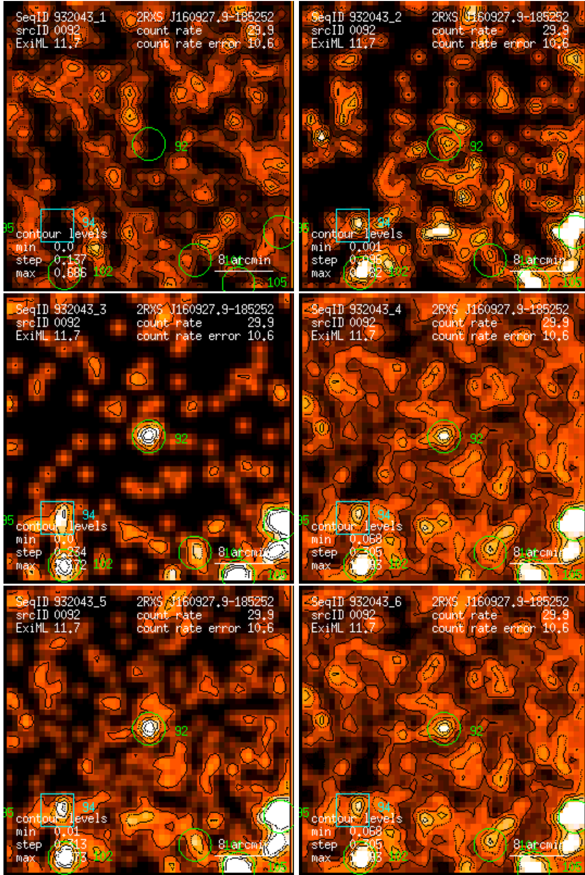
Figure 92: RASS 932043: detection 0092: band rate images, Gaussian filter: (1) PSPC channels 11 – 41, (2) 52 – 90, (3) 91 – 201, (4) 11 – 235, (5) 52 – 201, (6) 11 – 201. Broad band rates in counts/ks. Band rate contour levels in counts/ks/arcmin 2 .
