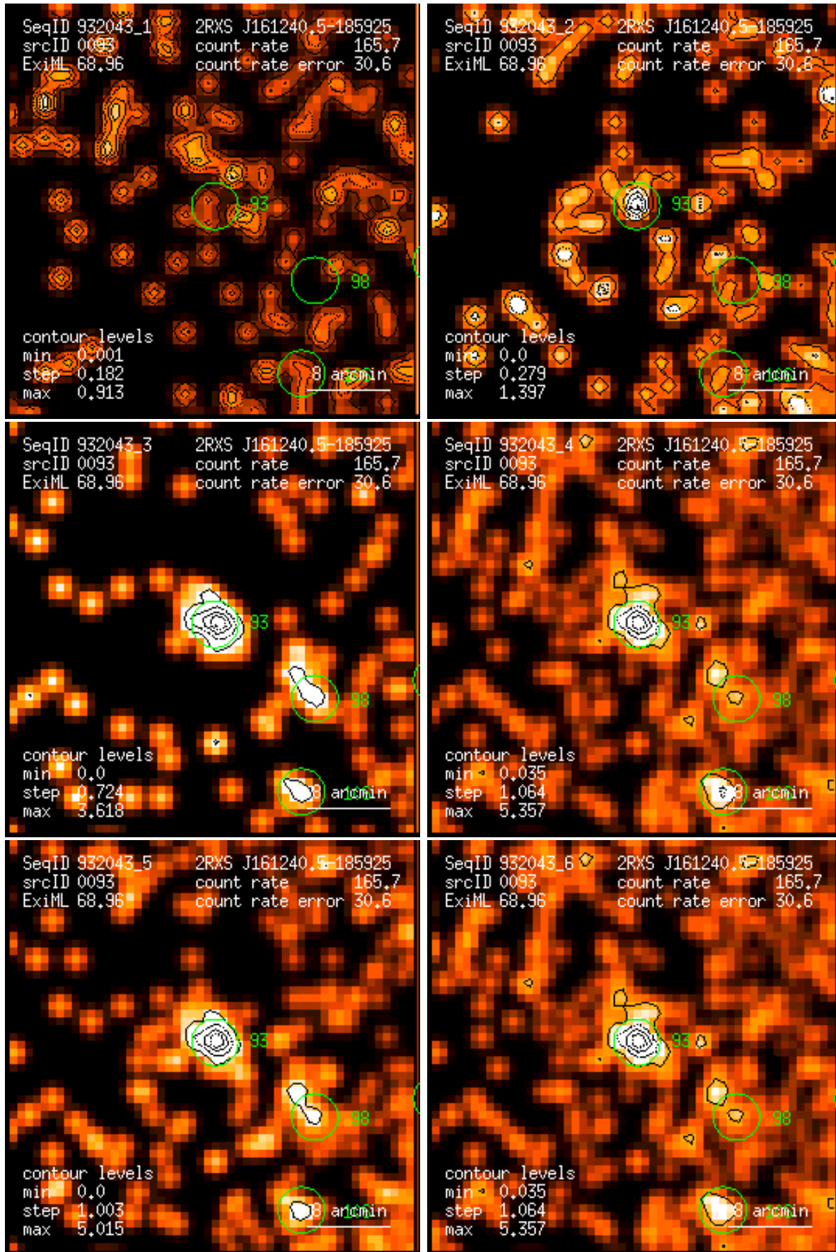
Figure 93: RASS 932043: detection 0093: band rate images, Gaussian filter: (1) PSPC channels 11 – 41, (2) 52 – 90, (3) 91 – 201, (4) 11 – 235, (5) 52 – 201, (6) 11 – 201. Broad band rates in counts/ks. Band rate contour levels in counts/ks/arcmin 2 .
