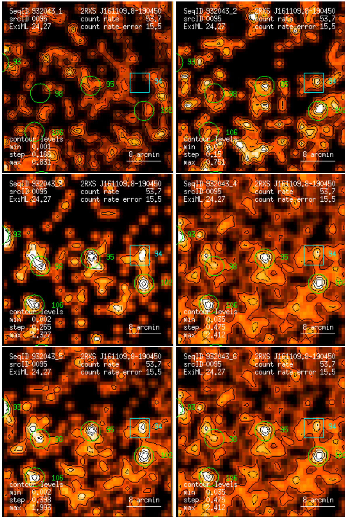
Figure 95: RASS 932043: detection 0095: band rate images, Gaussian filter: (1) PSPC channels 11 – 41, (2) 52 – 90, (3) 91 – 201, (4) 11 – 235, (5) 52 – 201, (6) 11 – 201. Broad band rates in counts/ks. Band rate contour levels in counts/ks/arcmin 2 .
