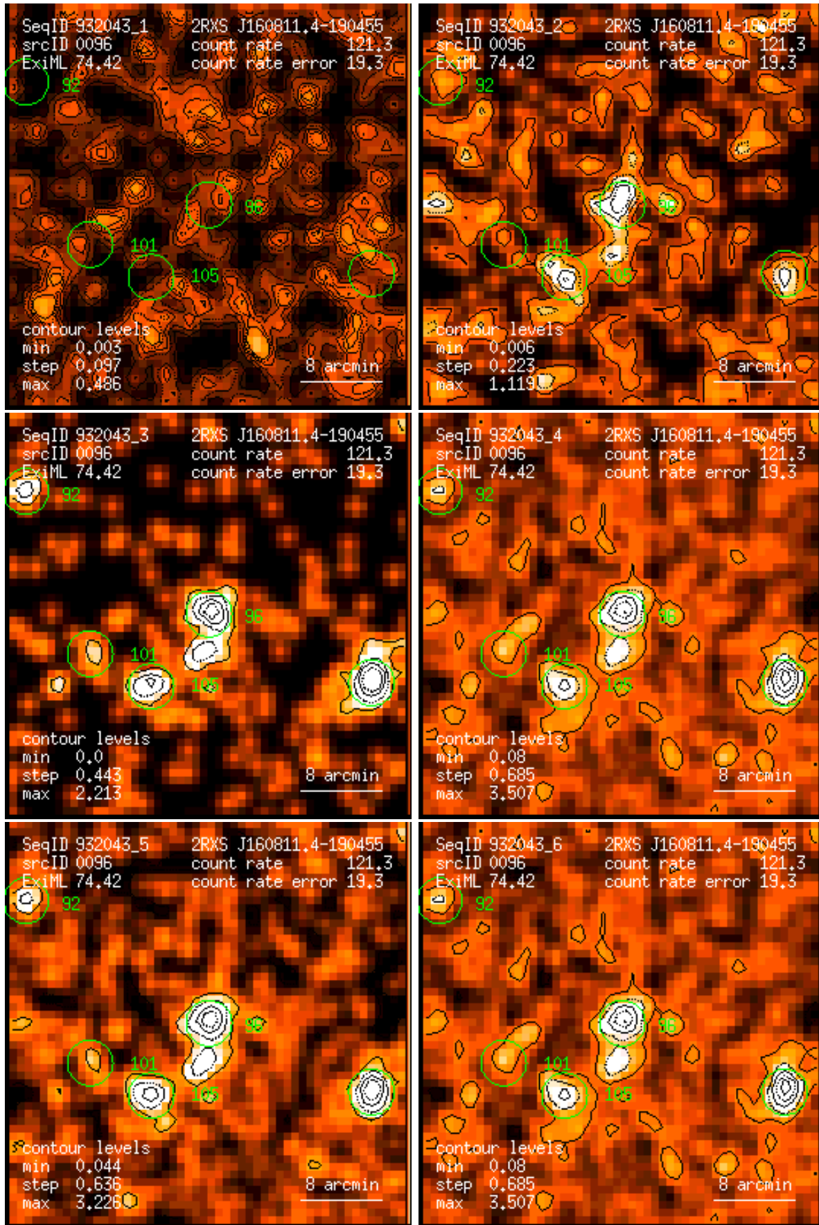
Figure 96: RASS 932043: detection 0096: band rate images, Gaussian filter: (1) PSPC channels 11 – 41, (2) 52 – 90, (3) 91 – 201, (4) 11 – 235, (5) 52 – 201, (6) 11 – 201. Broad band rates in counts/ks. Band rate contour levels in counts/ks/arcmin 2 .
