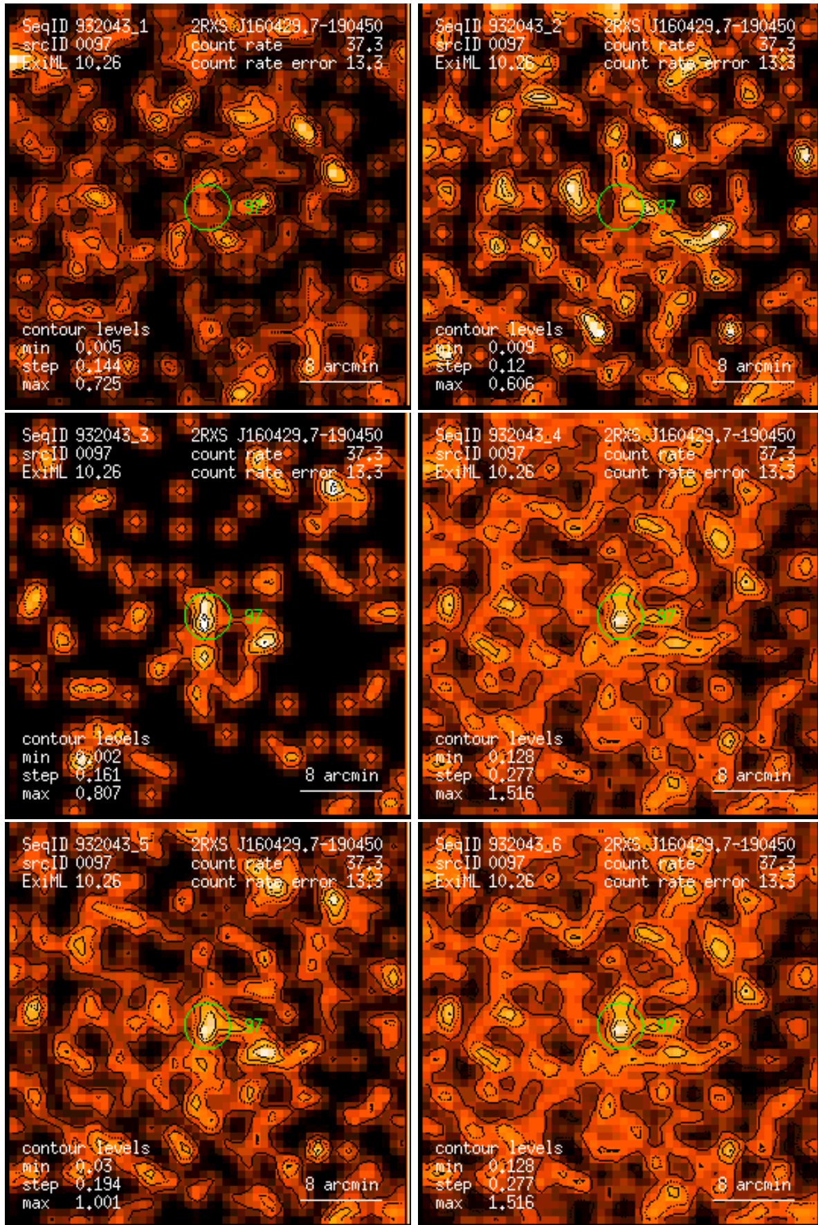
Figure 97: RASS 932043: detection 0097: band rate images, Gaussian filter: (1) PSPC channels 11 – 41, (2) 52 – 90, (3) 91 – 201, (4) 11 – 235, (5) 52 – 201, (6) 11 – 201. Broad band rates in counts/ks. Band rate contour levels in counts/ks/arcmin 2 .
