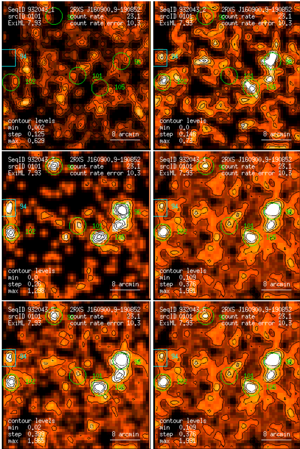
Figure 101: RASS 932043: detection 0101: band rate images, Gaussian filter: (1) PSPC channels 11 – 41, (2) 52 – 90, (3) 91 – 201, (4) 11 – 235, (5) 52 – 201, (6) 11 – 201. Broad band rates in counts/ks. Band rate contour levels in counts/ks/arcmin 2 .
