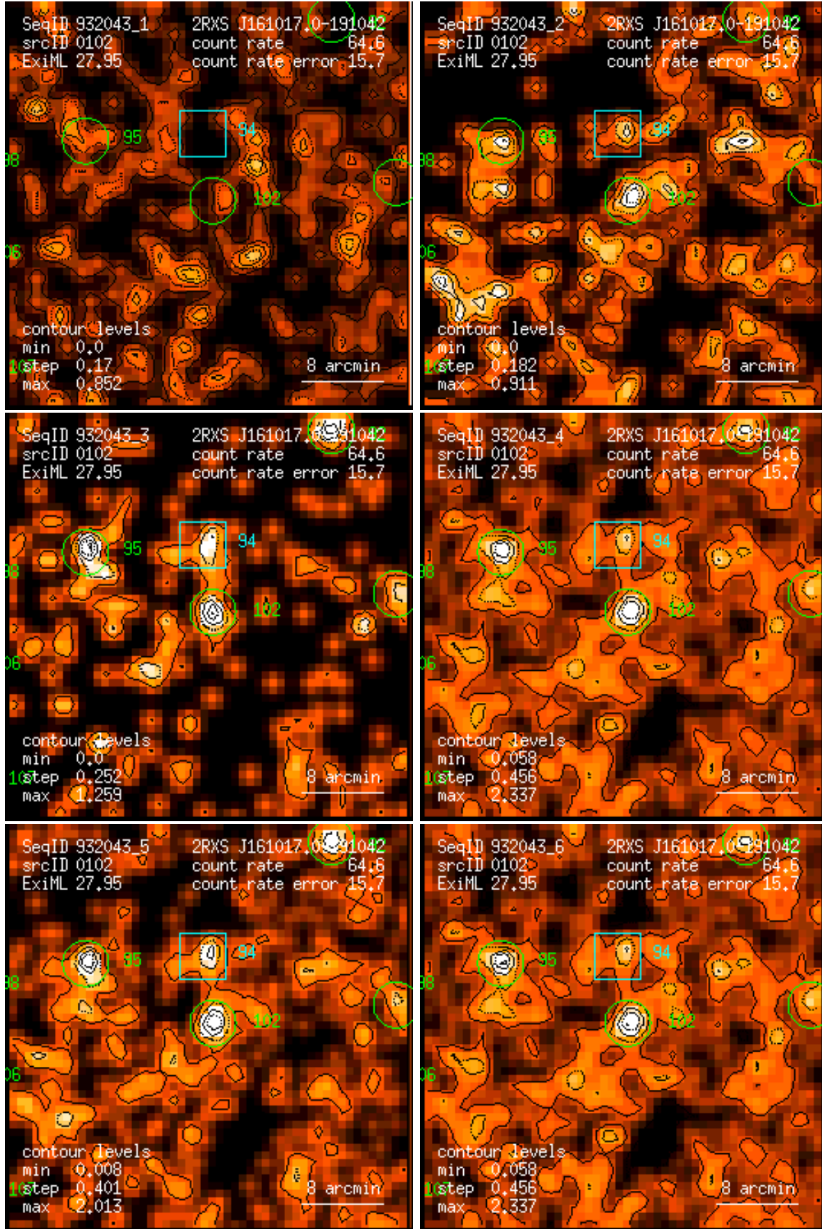
Figure 102: RASS 932043: detection 0102: band rate images, Gaussian filter: (1) PSPC channels 11 – 41, (2) 52 – 90, (3) 91 – 201, (4) 11 – 235, (5) 52 – 201, (6) 11 – 201. Broad band rates in counts/ks. Band rate contour levels in counts/ks/arcmin 2 .
