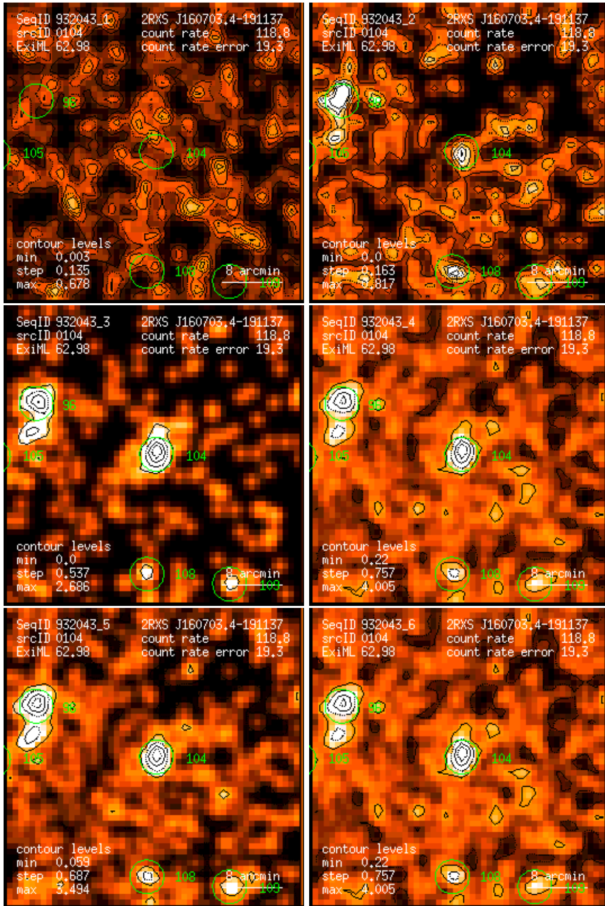
Figure 104: RASS 932043: detection 0104: band rate images, Gaussian filter: (1) PSPC channels 11 – 41, (2) 52 – 90, (3) 91 – 201, (4) 11 – 235, (5) 52 – 201, (6) 11 – 201. Broad band rates in counts/ks. Band rate contour levels in counts/ks/arcmin 2 .
