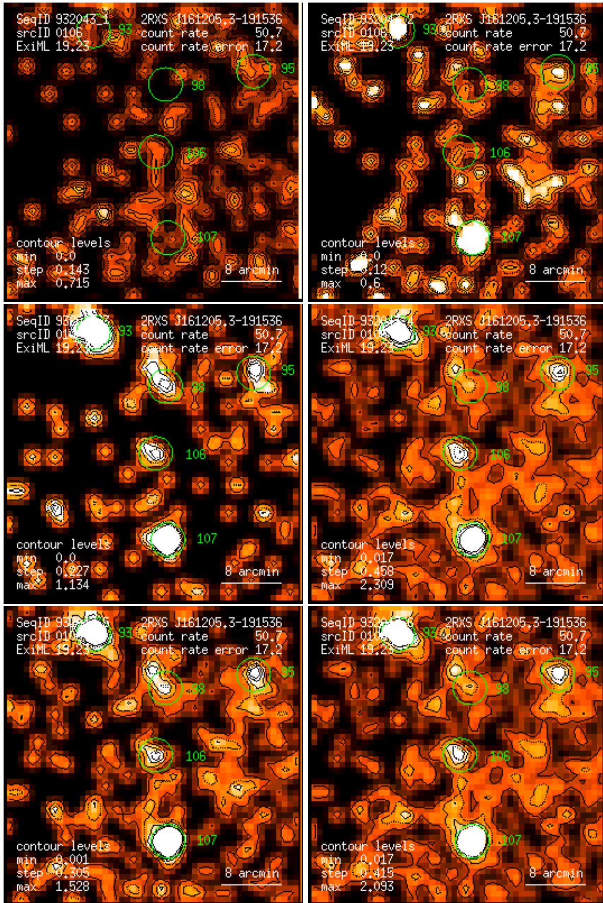
Figure 106: RASS 932043: detection 0106: band rate images, Gaussian filter: (1) PSPC channels 11 – 41, (2) 52 – 90, (3) 91 – 201, (4) 11 – 235, (5) 52 – 201, (6) 11 – 201. Broad band rates in counts/ks. Band rate contour levels in counts/ks/arcmin 2 .
