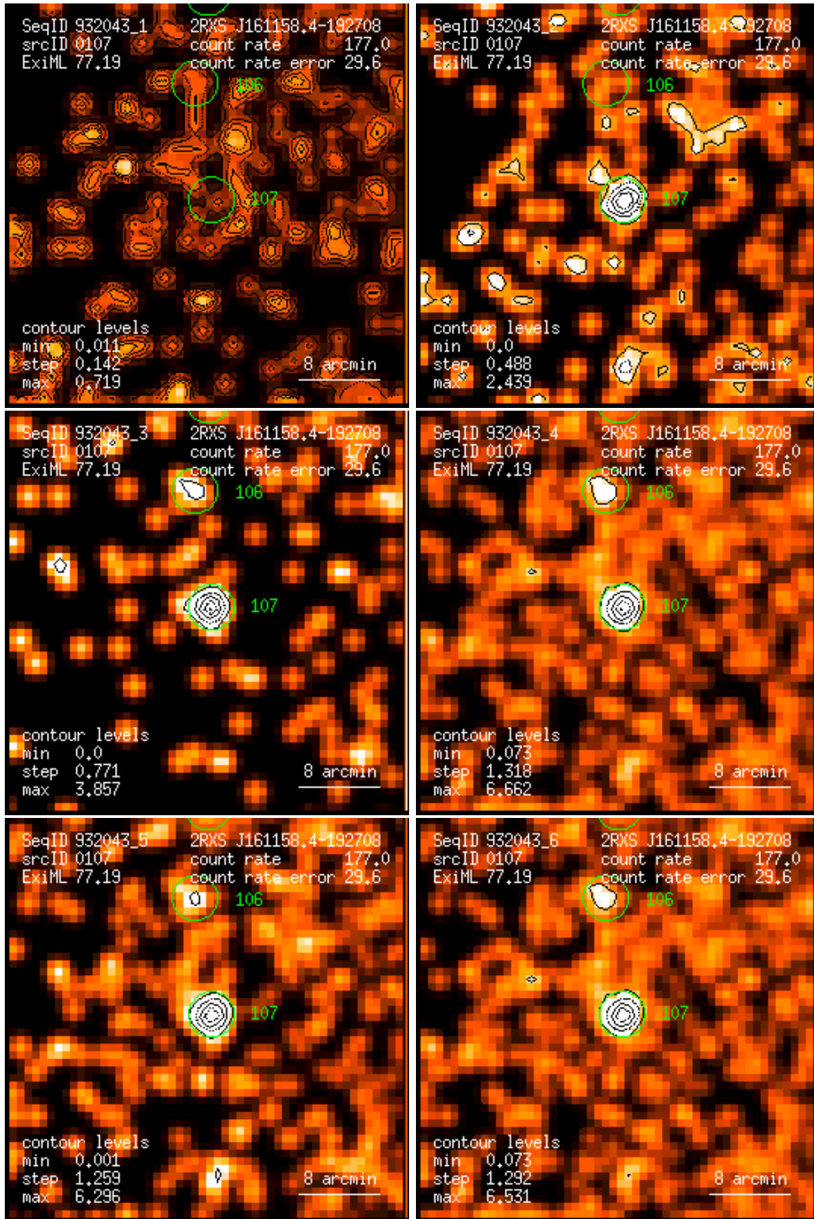
Figure 107: RASS 932043: detection 0107: band rate images, Gaussian filter: (1) PSPC channels 11 – 41, (2) 52 – 90, (3) 91 – 201, (4) 11 – 235, (5) 52 – 201, (6) 11 – 201. Broad band rates in counts/ks. Band rate contour levels in counts/ks/arcmin 2 .
