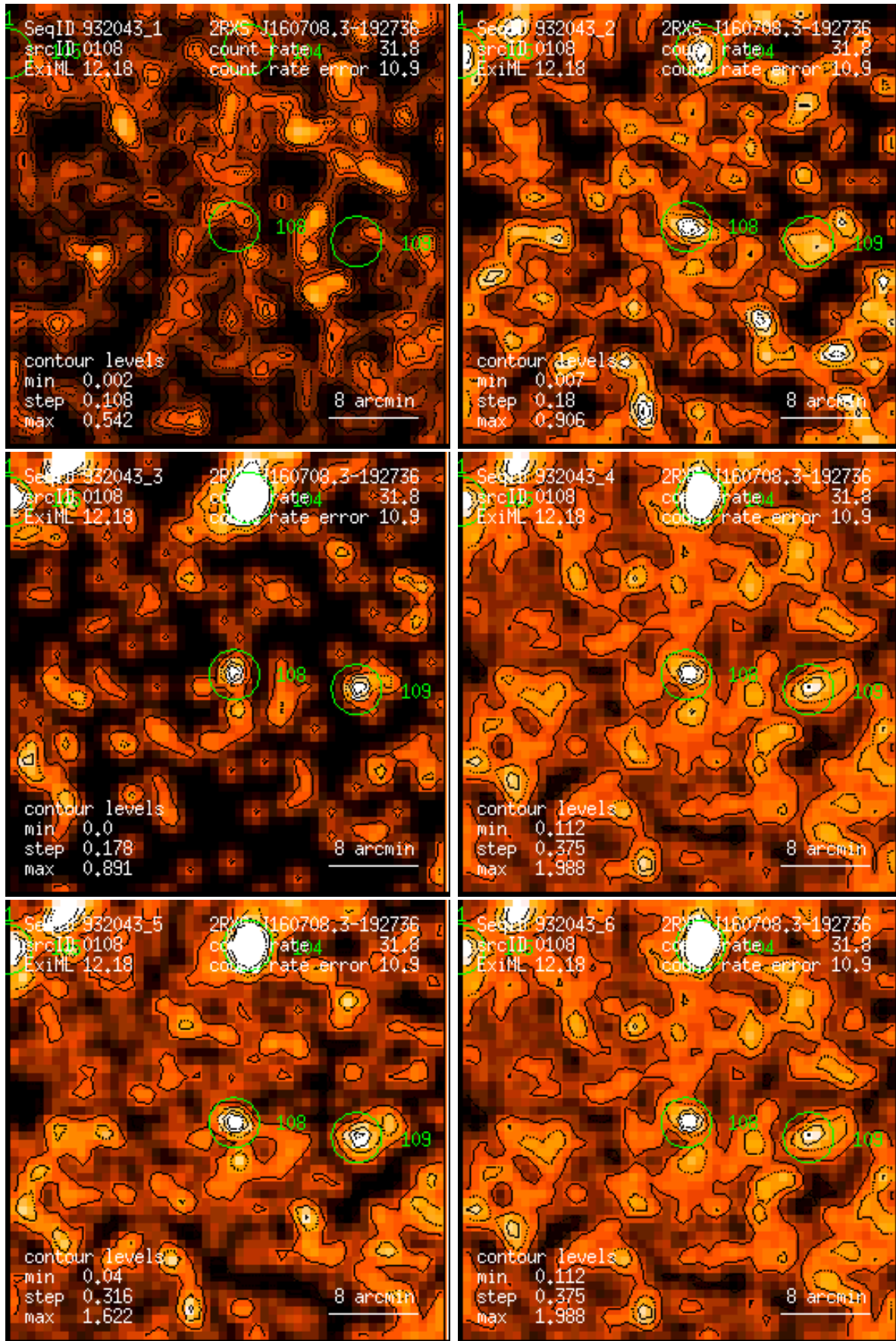
Figure 108: RASS 932043: detection 0108: band rate images, Gaussian filter: (1) PSPC channels 11 – 41, (2) 52 – 90, (3) 91 – 201, (4) 11 – 235, (5) 52 – 201, (6) 11 – 201. Broad band rates in counts/ks. Band rate contour levels in counts/ks/arcmin 2 .
