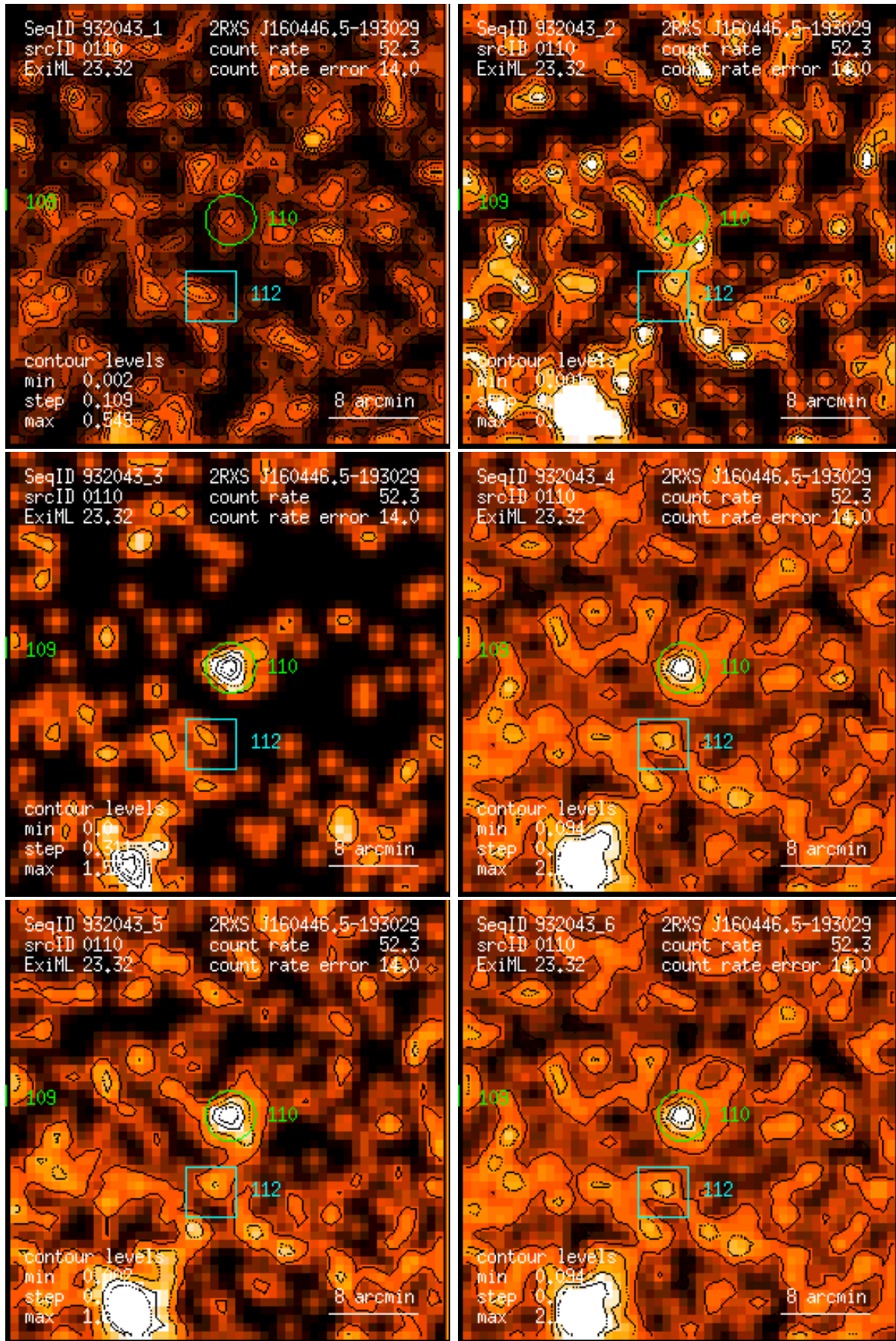
Figure 110: RASS 932043: detection 0110: band rate images, Gaussian filter: (1) PSPC channels 11 – 41, (2) 52 – 90, (3) 91 – 201, (4) 11 – 235, (5) 52 – 201, (6) 11 – 201. Broad band rates in counts/ks. Band rate contour levels in counts/ks/arcmin 2 .
