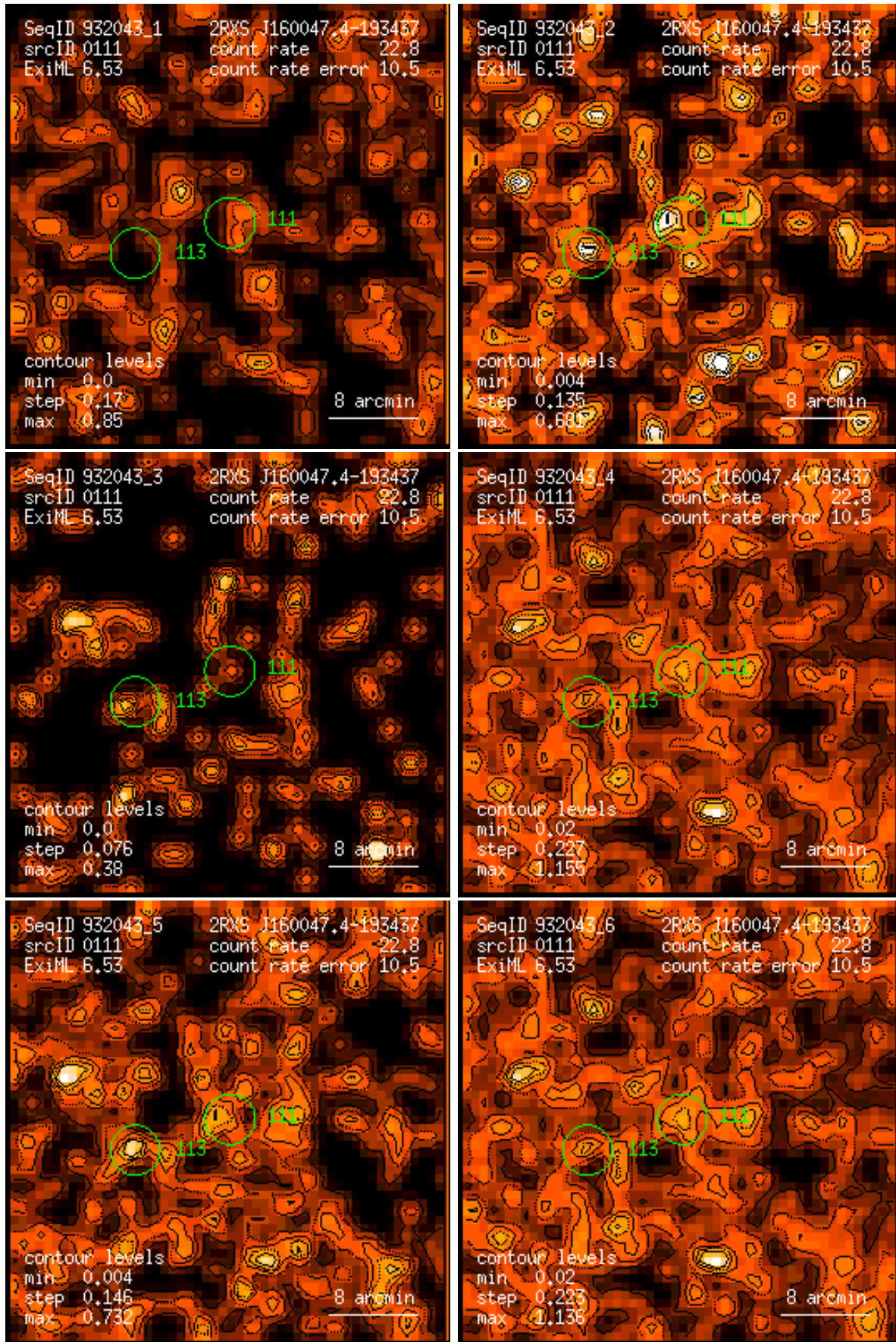
Figure 111: RASS 932043: detection 0111: band rate images, Gaussian filter: (1) PSPC channels 11 – 41, (2) 52 – 90, (3) 91 – 201, (4) 11 – 235, (5) 52 – 201, (6) 11 – 201. Broad band rates in counts/ks. Band rate contour levels in counts/ks/arcmin 2 .
