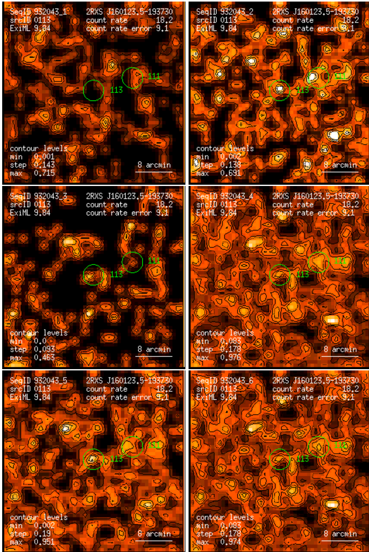
Figure 113: RASS 932043: detection 0113: band rate images, Gaussian filter: (1) PSPC channels 11 – 41, (2) 52 – 90, (3) 91 – 201, (4) 11 – 235, (5) 52 – 201, (6) 11 – 201. Broad band rates in counts/ks. Band rate contour levels in counts/ks/arcmin 2 .
