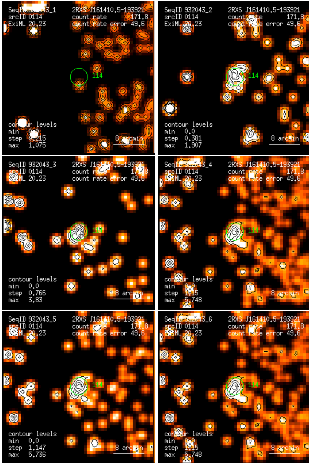
Figure 114: RASS 932043: detection 0114: band rate images, Gaussian filter: (1) PSPC channels 11 – 41, (2) 52 – 90, (3) 91 – 201, (4) 11 – 235, (5) 52 – 201, (6) 11 – 201. Broad band rates in counts/ks. Band rate contour levels in counts/ks/arcmin 2 .
