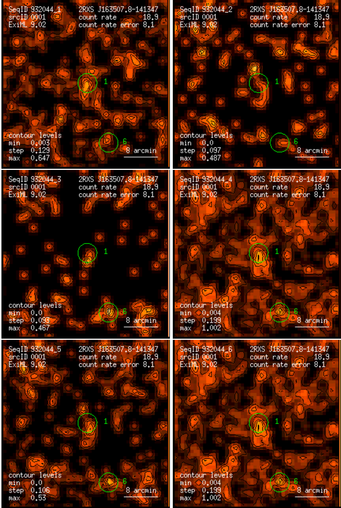
Figure 1: RASS 932044: detection 0001: band rate images, Gaussian filter: (1) PSPC channels 11 – 41, (2) 52 – 90, (3) 91 – 201, (4) 11 – 235, (5) 52 – 201, (6) 11 – 201. Broad band rates in counts/ks. Band rate contour levels in counts/ks/arcmin 2 .
