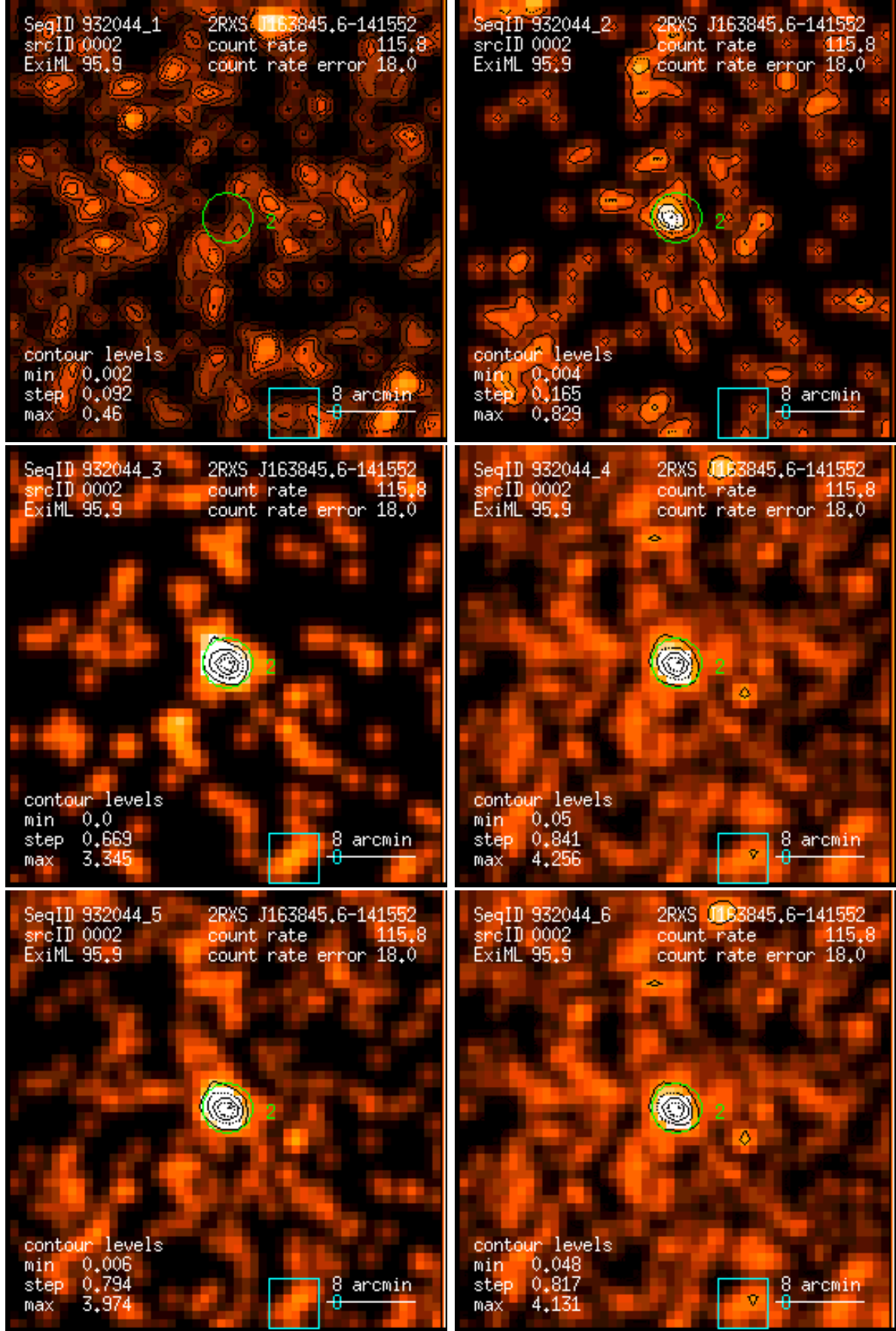
Figure 2: RASS 932044: detection 0002: band rate images, Gaussian filter: (1) PSPC channels 11 – 41, (2) 52 – 90, (3) 91 – 201, (4) 11 – 235, (5) 52 – 201, (6) 11 – 201. Broad band rates in counts/ks. Band rate contour levels in counts/ks/arcmin 2 .
