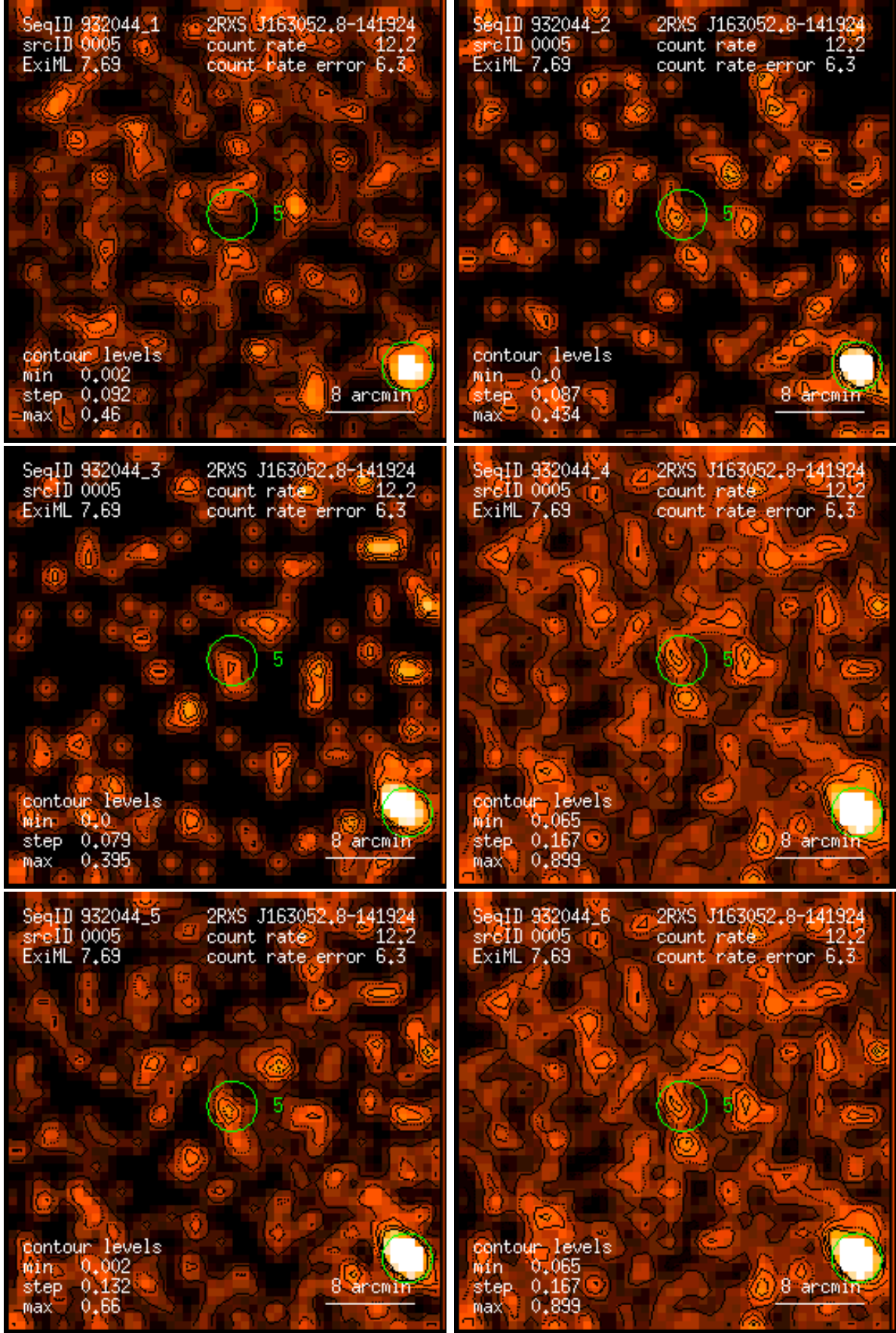
Figure 5: RASS 932044: detection 0005: band rate images, Gaussian filter: (1) PSPC channels 11 – 41, (2) 52 – 90, (3) 91 – 201, (4) 11 – 235, (5) 52 – 201, (6) 11 – 201. Broad band rates in counts/ks. Band rate contour levels in counts/ks/arcmin 2 .
