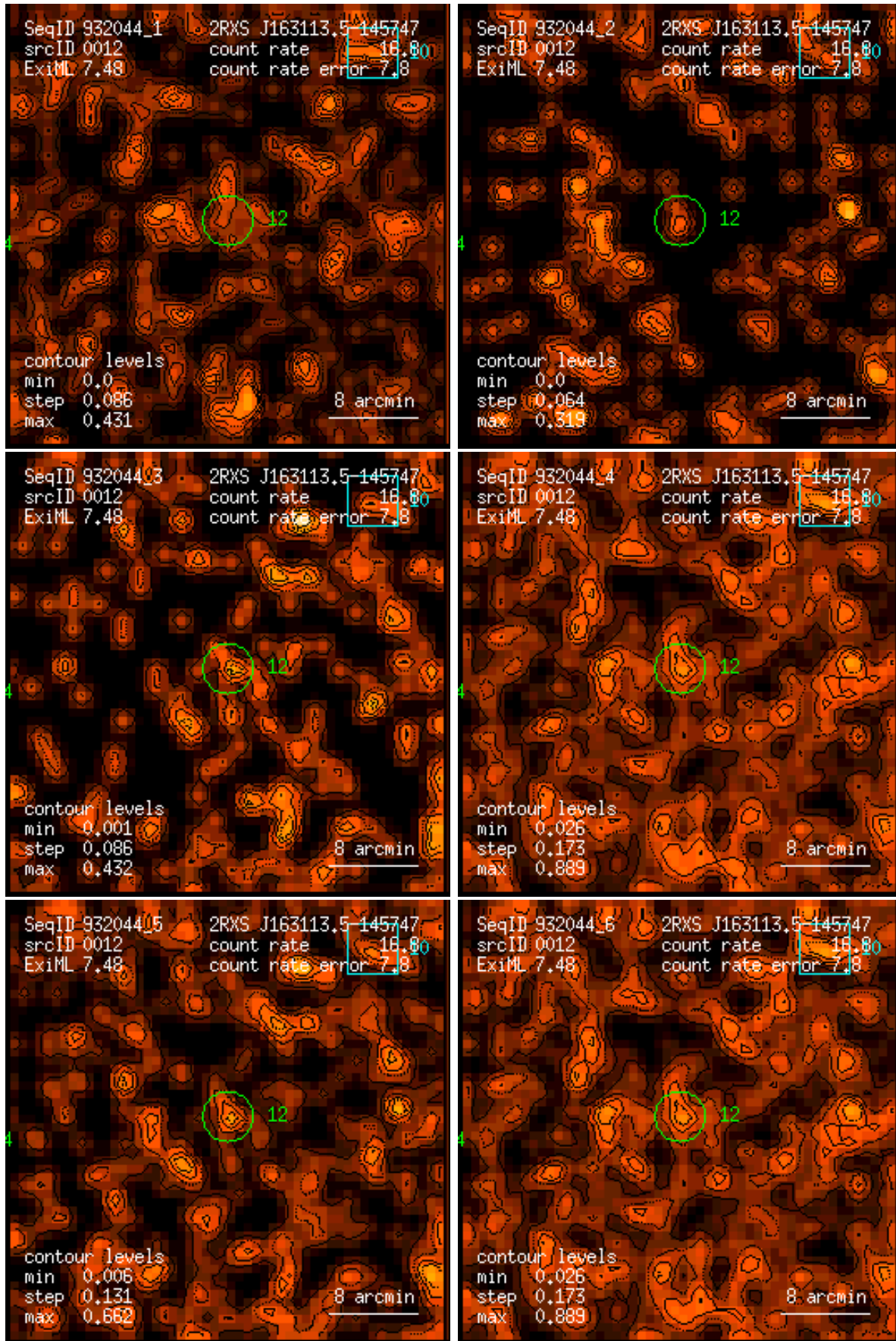
Figure 12: RASS 932044: detection 0012: band rate images, Gaussian filter: (1) PSPC channels 11 – 41, (2) 52 – 90, (3) 91 – 201, (4) 11 – 235, (5) 52 – 201, (6) 11 – 201. Broad band rates in counts/ks. Band rate contour levels in counts/ks/arcmin 2 .
