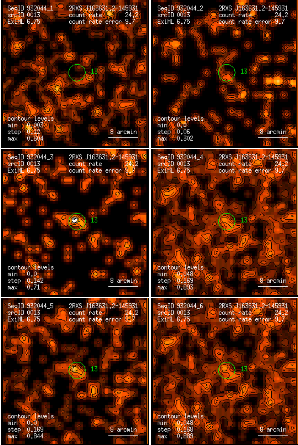
Figure 13: RASS 932044: detection 0013: band rate images, Gaussian filter: (1) PSPC channels 11 – 41, (2) 52 – 90, (3) 91 – 201, (4) 11 – 235, (5) 52 – 201, (6) 11 – 201. Broad band rates in counts/ks. Band rate contour levels in counts/ks/arcmin 2 .
