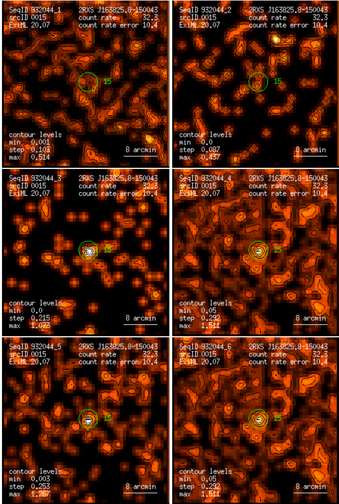
Figure 15: RASS 932044: detection 0015: band rate images, Gaussian filter: (1) PSPC channels 11 – 41, (2) 52 – 90, (3) 91 – 201, (4) 11 – 235, (5) 52 – 201, (6) 11 – 201. Broad band rates in counts/ks. Band rate contour levels in counts/ks/arcmin 2 .
