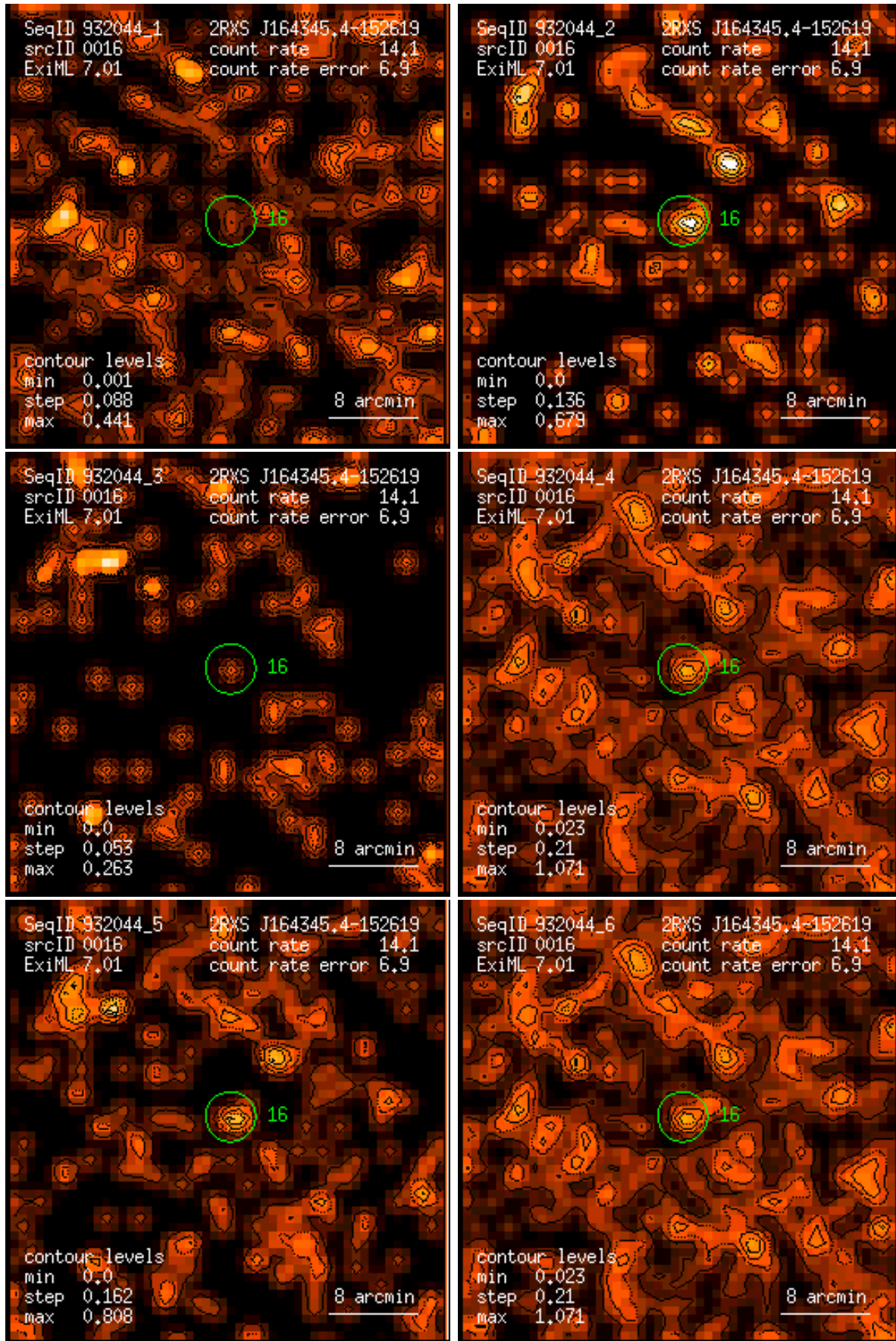
Figure 16: RASS 932044: detection 0016: band rate images, Gaussian filter: (1) PSPC channels 11 – 41, (2) 52 – 90, (3) 91 – 201, (4) 11 – 235, (5) 52 – 201, (6) 11 – 201. Broad band rates in counts/ks. Band rate contour levels in counts/ks/arcmin 2 .
