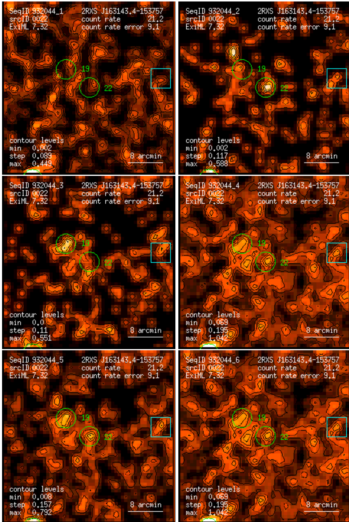
Figure 22: RASS 932044: detection 0022: band rate images, Gaussian filter: (1) PSPC channels 11 – 41, (2) 52 – 90, (3) 91 – 201, (4) 11 – 235, (5) 52 – 201, (6) 11 – 201. Broad band rates in counts/ks. Band rate contour levels in counts/ks/arcmin 2 .
