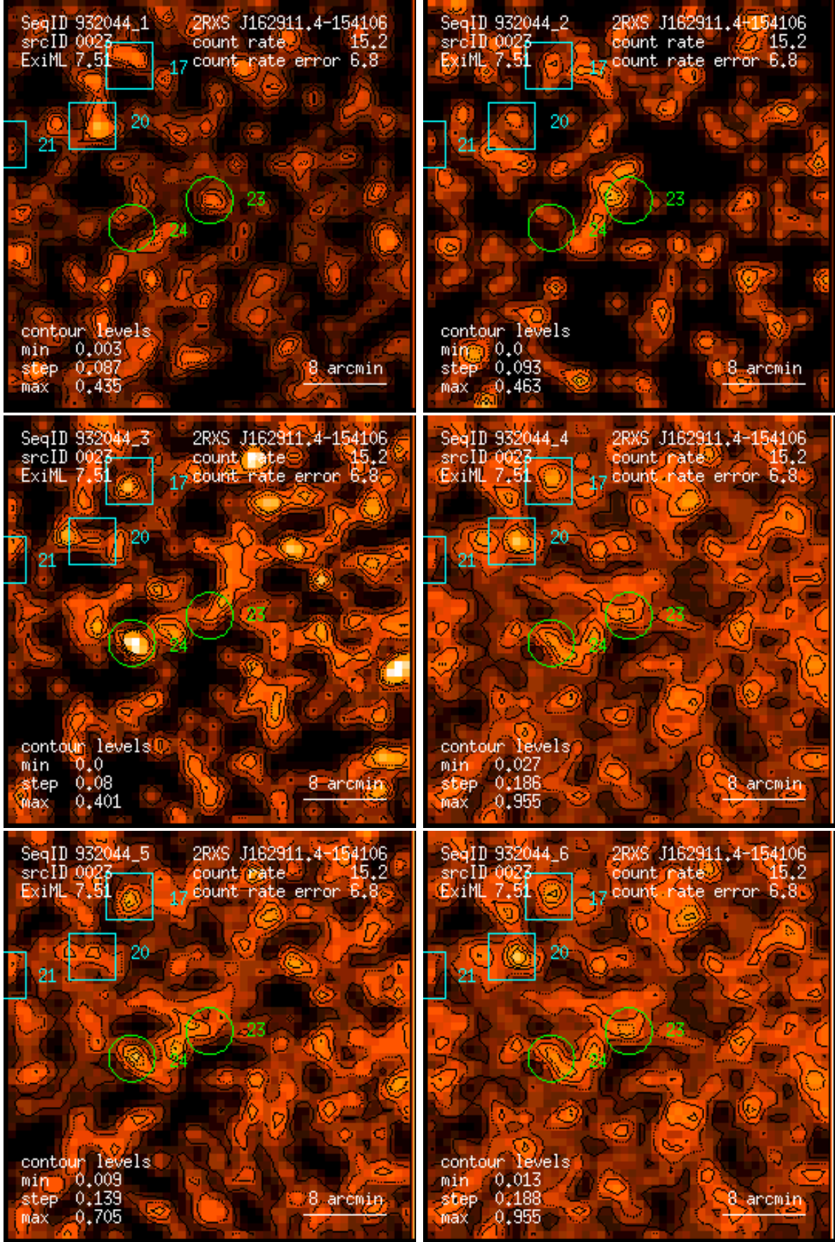
Figure 23: RASS 932044: detection 0023: band rate images, Gaussian filter: (1) PSPC channels 11 – 41, (2) 52 – 90, (3) 91 – 201, (4) 11 – 235, (5) 52 – 201, (6) 11 – 201. Broad band rates in counts/ks. Band rate contour levels in counts/ks/arcmin 2 .
