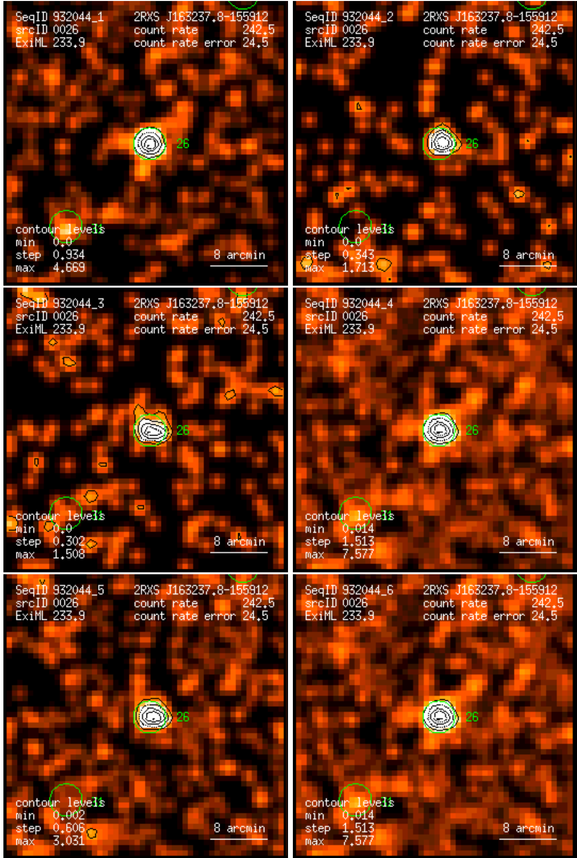
Figure 26: RASS 932044: detection 0026: band rate images, Gaussian filter: (1) PSPC channels 11 – 41, (2) 52 – 90, (3) 91 – 201, (4) 11 – 235, (5) 52 – 201, (6) 11 – 201. Broad band rates in counts/ks. Band rate contour levels in counts/ks/arcmin 2 .
