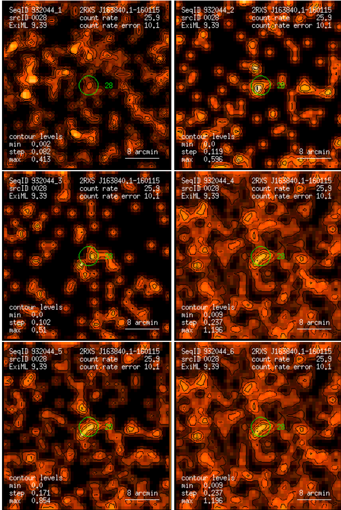
Figure 28: RASS 932044: detection 0028: band rate images, Gaussian filter: (1) PSPC channels 11 – 41, (2) 52 – 90, (3) 91 – 201, (4) 11 – 235, (5) 52 – 201, (6) 11 – 201. Broad band rates in counts/ks. Band rate contour levels in counts/ks/arcmin 2 .
