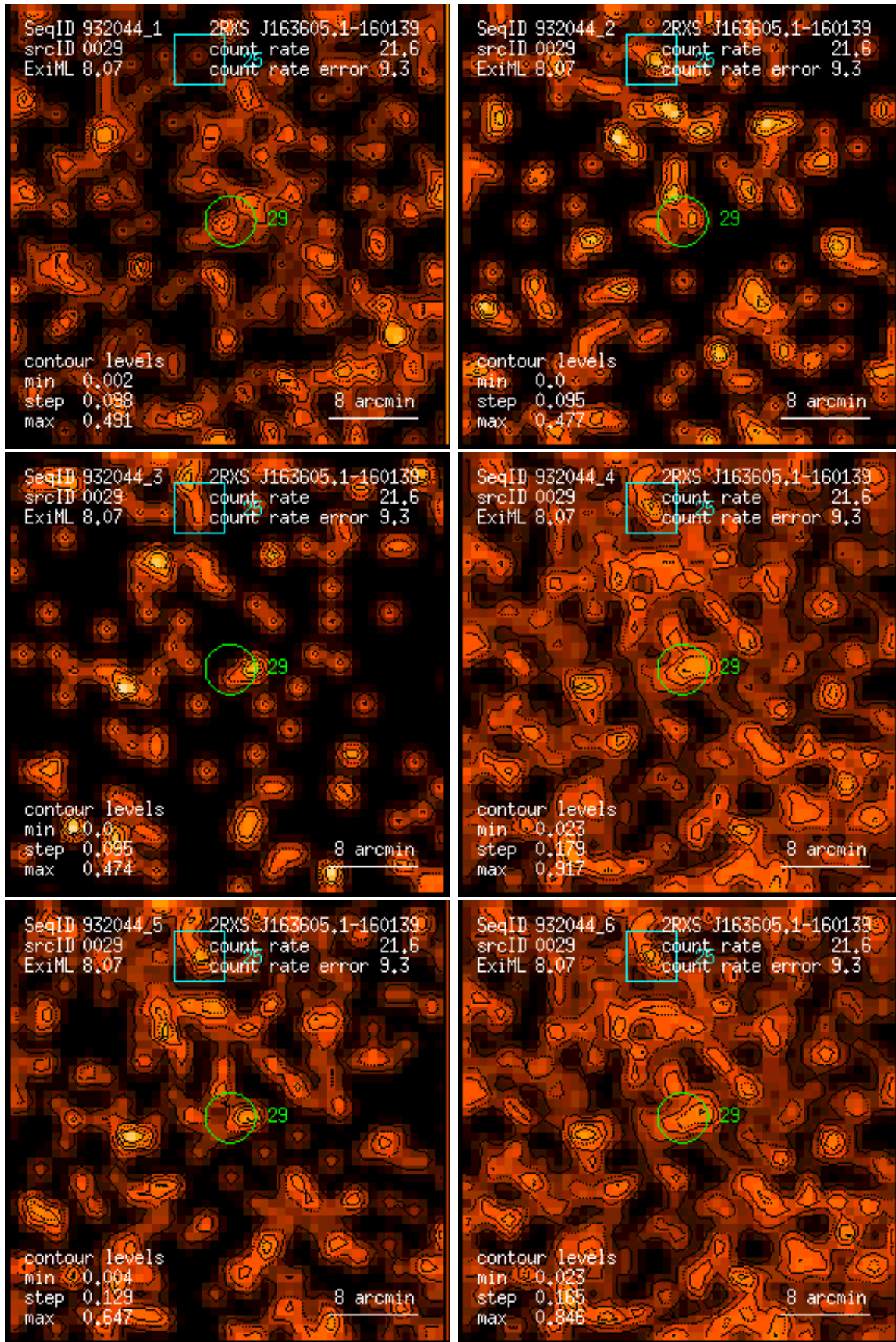
Figure 29: RASS 932044: detection 0029: band rate images, Gaussian filter: (1) PSPC channels 11 – 41, (2) 52 – 90, (3) 91 – 201, (4) 11 – 235, (5) 52 – 201, (6) 11 – 201. Broad band rates in counts/ks. Band rate contour levels in counts/ks/arcmin 2 .
