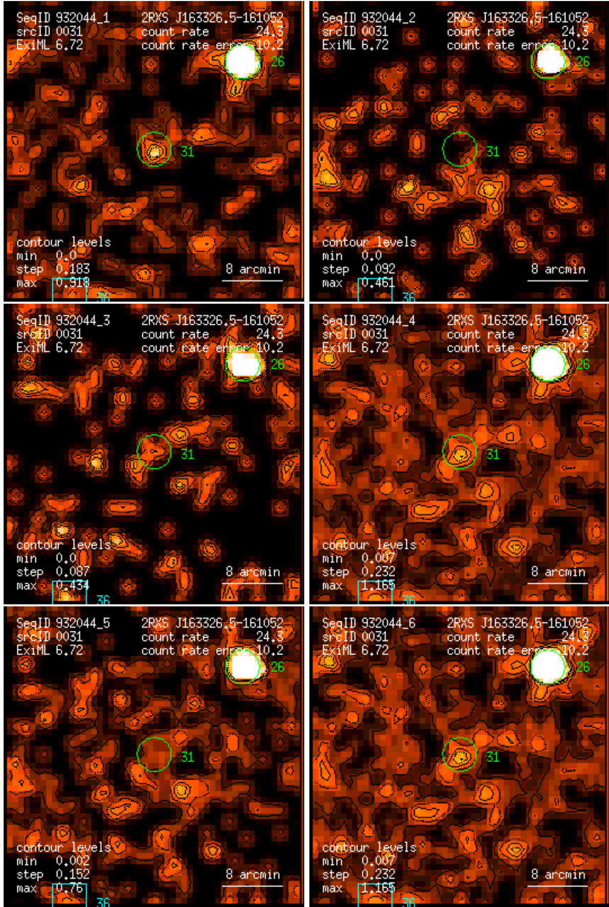
Figure 31: RASS 932044: detection 0031: band rate images, Gaussian filter: (1) PSPC channels 11 – 41, (2) 52 – 90, (3) 91 – 201, (4) 11 – 235, (5) 52 – 201, (6) 11 – 201. Broad band rates in counts/ks. Band rate contour levels in counts/ks/arcmin 2 .
