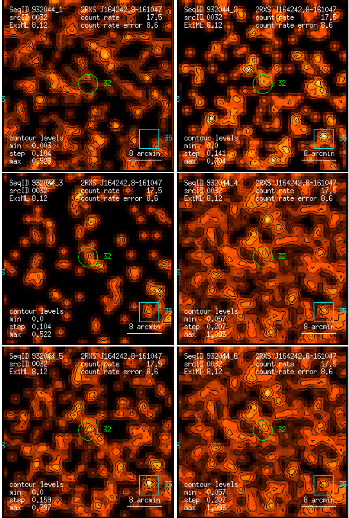
Figure 32: RASS 932044: detection 0032: band rate images, Gaussian filter: (1) PSPC channels 11 – 41, (2) 52 – 90, (3) 91 – 201, (4) 11 – 235, (5) 52 – 201, (6) 11 – 201. Broad band rates in counts/ks. Band rate contour levels in counts/ks/arcmin 2 .
