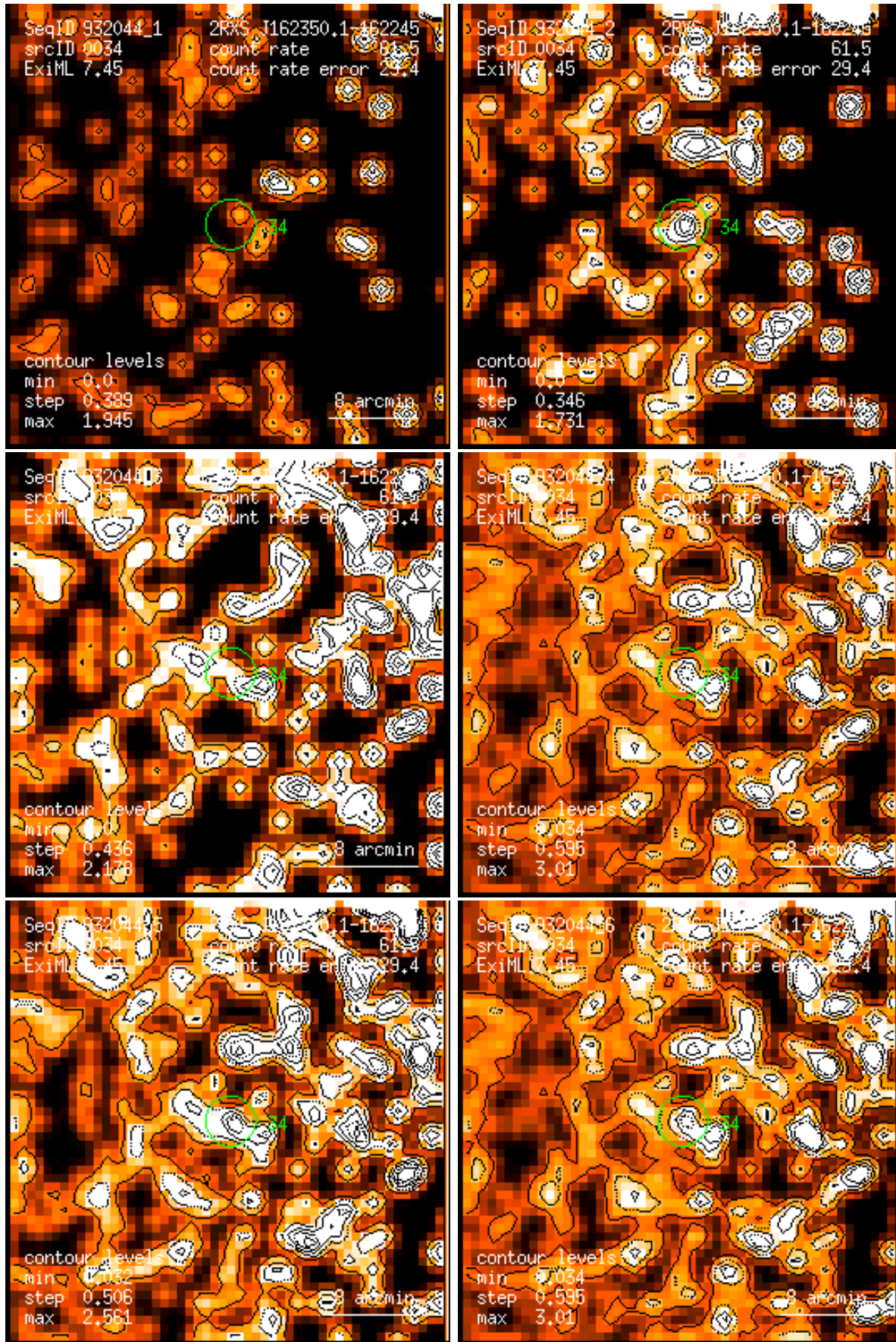
Figure 34: RASS 932044: detection 0034: band rate images, Gaussian filter: (1) PSPC channels 11 – 41, (2) 52 – 90, (3) 91 – 201, (4) 11 – 235, (5) 52 – 201, (6) 11 – 201. Broad band rates in counts/ks. Band rate contour levels in counts/ks/arcmin 2 .
