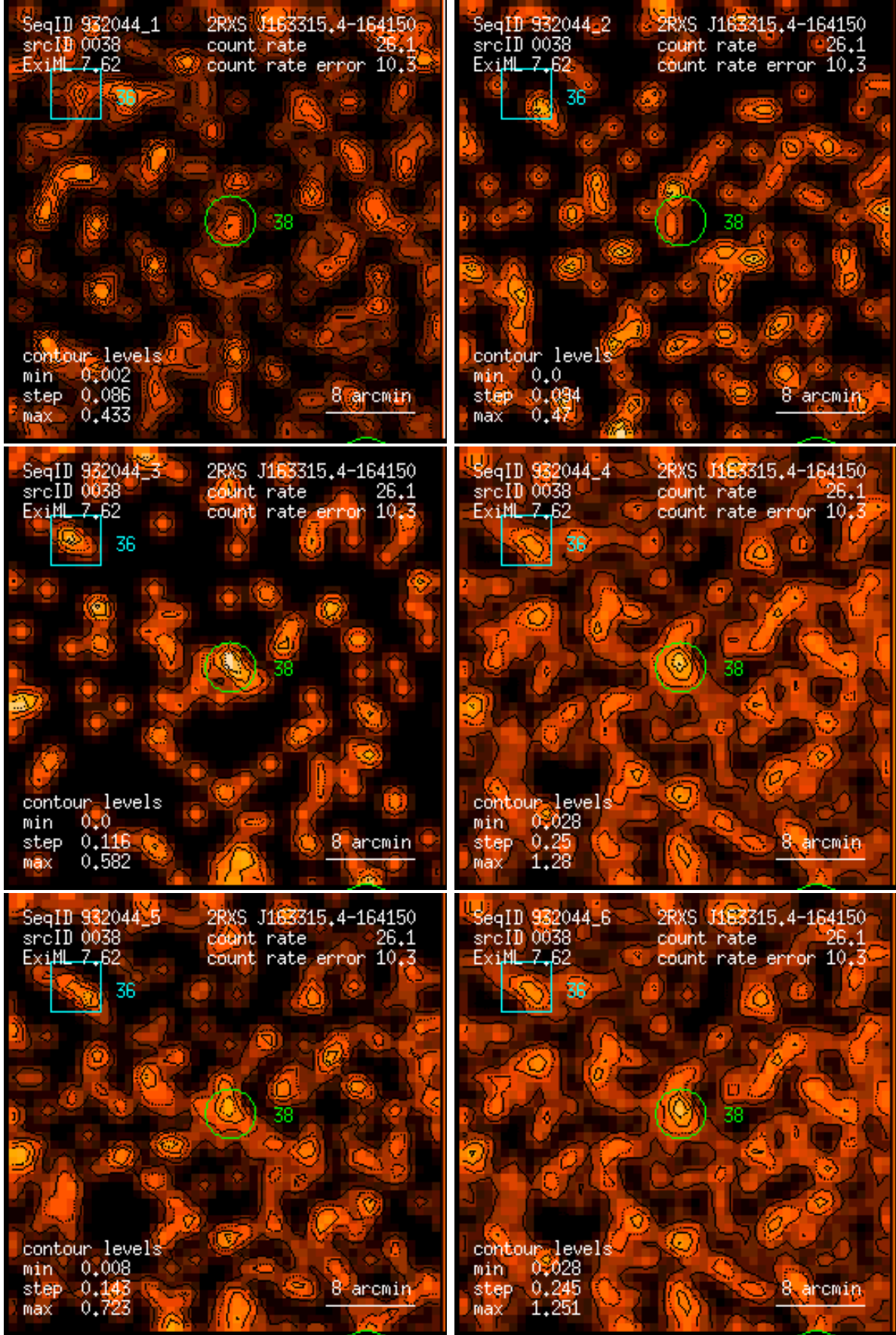
Figure 38: RASS 932044: detection 0038: band rate images, Gaussian filter: (1) PSPC channels 11 – 41, (2) 52 – 90, (3) 91 – 201, (4) 11 – 235, (5) 52 – 201, (6) 11 – 201. Broad band rates in counts/ks. Band rate contour levels in counts/ks/arcmin 2 .
