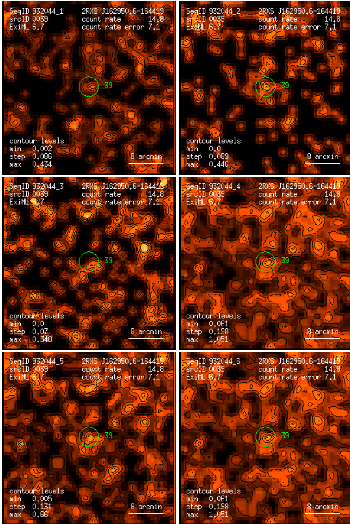
Figure 39: RASS 932044: detection 0039: band rate images, Gaussian filter: (1) PSPC channels 11 – 41, (2) 52 – 90, (3) 91 – 201, (4) 11 – 235, (5) 52 – 201, (6) 11 – 201. Broad band rates in counts/ks. Band rate contour levels in counts/ks/arcmin 2 .
